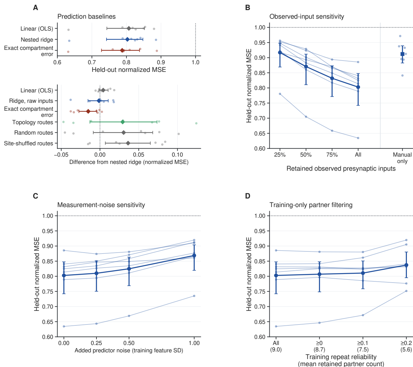
Figure S32: Linear baselines explain most measured-response prediction, and degrading observed inputs worsens performance. Thirteen scans retain the complete-tree analysis's 130 outer stimulus-identity splits. All preprocessing, reliability masks and ridge tuning use training identities only. A , Ordinary least-squares (OLS) and nested ridge-regression baselines against the archived exact compartment-error fit; the dotted line is the training-mean predictor (normalized MSE = 1 by construction). Lower normalized MSE is better. Below, paired differences from nested ridge (dotted line, zero difference) for each comparator: OLS, ridge on untransformed inputs, the exact compartment-error fit, and the archived route-restricted fits with topology-matched (ancestry), random anatomical and site-shuffled routes, whose absolute errors are in Supplementary Fig. S31C. The exact fit gives a small additional nonlinear benefit, mean -0.0152 (95% interval -0.0271 to -0.0042 ), whereas topology-matched routes ( 0.029 ; -0.013 to 0.074 ) are matched by random routes ( 0.031 ; -0.009 to 0.068 ). B , Ridge prediction when retaining nested random fractions of observed presynaptic inputs; five masks per split are averaged before inference. Manual-only partners, right of the separator, are the same ridge model under a provenance restriction, not a random retention dose. Empty masks use the training mean and remain included. C , Added Gaussian predictor noise in both training and test data, in units of training input standard deviation (SD) after the quantile transform. D , Reliability filtering based only on training repeats; parentheses give mean retained partner counts. In B–D the dotted horizontal line marks the training-mean predictor (normalized MSE = 1). Thin traces and small dots show seven target means after averaging splits within scan and scans within target. Larger symbols and bars are means and 95% target-bootstrap intervals (20,000 draws). All targets come from one mouse. Only ridge is refitted under the sensitivity conditions. Removing observed inputs does not recover unknown partners, establish population power or explain away the absence of preferential ancestry alignment.
