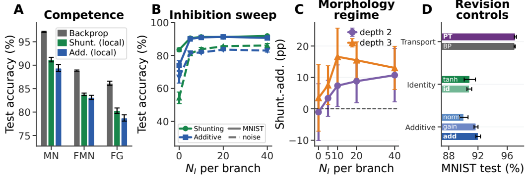
Figure 4: Capacity-calibrated competence and regime dependence. (A) Matched backprop vs. per-soma 5F LocalCA on MNIST, Fashion-MNIST, and figure-ground MNIST. (B) Inhibitory dose-response. (C) Morphology-dependent shunting advantage on noise resilience. (D) MNIST revision controls: BP = matched shunting backprop, PT = exact path-transported-error LocalCA, tanh/id = post-voltage param_tanh vs. identity upward transfer, and add/gain/norm = plain additive, best additive-gain, and best normalized-additive controls. Error bars denote \pm 1 s.d. where available.
