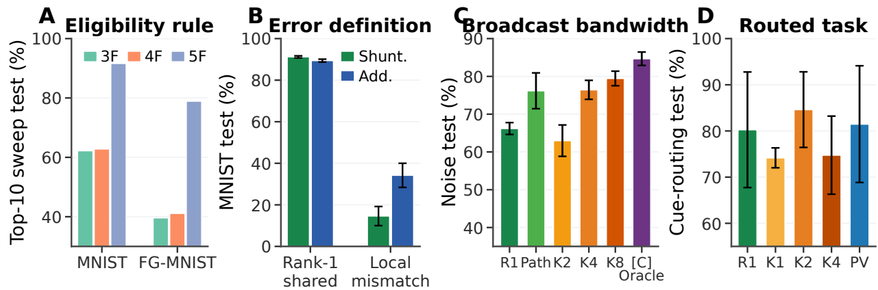
Figure S1: Detailed rule and feedback controls. (A) Eligibility-rule ablation: 3F, 4F, and 5F. (B) Error-source ablation: soma-derived feedback vs. local mismatch. (C) Feedback-bandwidth ladder on noise resilience: per-soma, recursive Path, K2/K4/K8, and [C] transported Oracle. (D) Cue routing: scalar/per-soma, random low-rank K1/K2/K4, and pathway-vector feedback.
