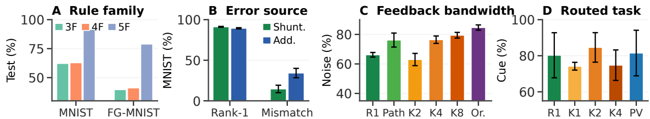
Figure 5: Rule and feedback controls. (A) Eligibility-rule ablation: 3F and 4F learn weakly, while 5F is the practical LocalCA rule. (B) Error-source ablation: Rank-1 = soma-derived shared feedback, and Mismatch = local-mismatch heuristic. (C) Noise-resilience feedback ladder: R1 = restricted per-soma/shared baseline, Path = recursive path-propagation proxy, K2/K4/K8 = random low-rank broadcast rank, and Or. = exact transported-error oracle. (D) Cue-routing rank diagnostic: R1 = restricted baseline, K1/K2/K4 = random low-rank ranks, and PV = pathway-vector feedback.
