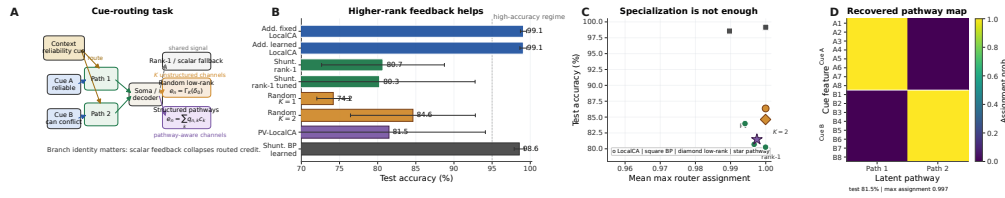
Figure S17: Structured feedback when rank-1 broadcast fails. (A) Cue-routing task schematic. Context determines which noisy cue is reliable on each trial, so different dendritic pathways should receive different teaching signals. (B) Five-seed comparison of rank-1, random low-rank, and pathway-structured feedback. Moving beyond rank-1 helps, while the best structured repair remains open. (C) Test accuracy vs. router specialization across learned-router conditions. High specialization alone does not guarantee success. (D) Recovered pathway assignments for a representative learned-router run. Cue-A and cue-B features segregate into separate latent pathways even when feedback quality, rather than router discreteness, is the limiting factor.
