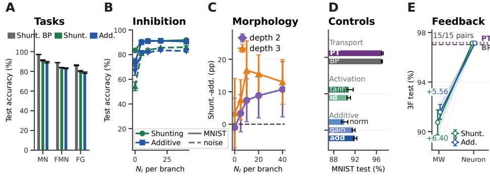
Figure 4: Matched-capacity performance, regime dependence, and feedback definition. (A) Matched shunting backpropagation reference (grey, labelled Shunt. BP) vs. 5F LocalCA with matched-width/scalar-fallback feedback; MN, FMN, and FG denote MNIST, Fashion-MNIST, and figure-ground MNIST. Additive backpropagation references are reported in Table S8 where matched five-seed runs are available. (B) Inhibitory dose-response. (C) Descriptive morphology-by-inhibition performance; the detailed map and its initialization limitation are in Appendix Fig. S10. (D) MNIST controls: BP and exact path transport (PT); learned tanh versus identity transfer (id.); normalized eligibility (+norm); gain-matched additive eligibility (gain); and the additive core (add.). (E) Fifteen-seed 3F intervention: replacing matched-width/scalar-fallback feedback (MW) by one neuron-indexed coordinate shared within each modeled tree raises accuracy by 6.40 points in shunting and 5.56 points in additive networks; all paired seeds improve. Dashed and dotted lines mark the matched shunting BP and exact-transport references. Values/protocols: Table S8; Appendix A. Error bars denote \pm 1 s.d.
