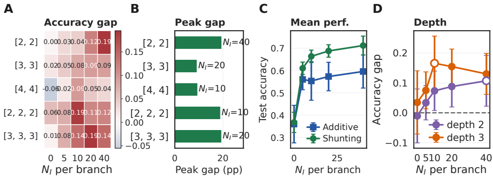
Figure S10: Descriptive morphology \times inhibition performance map. (A) Shunting-minus-additive LocalCA accuracy gap across dendritic morphologies and inhibitory synapse counts. (B) Best inhibitory count for each morphology. (C) Mean performance across tested trees. (D) Average shunting advantage by depth, with markers showing the peak inhibitory count for each depth. The grid uses nonnegative inputs. Because analytical initialization places one shunting population at a near-zero coupling floor, these comparisons are descriptive rather than a causal morphology intervention.
