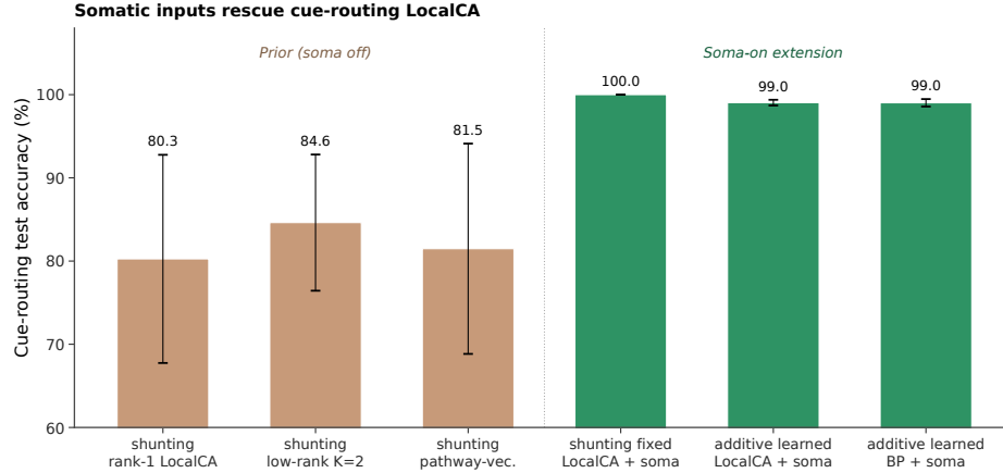
Figure S12: Soma-on rescues cue-routing LocalCA. The left bars show the previously reported soma-off LocalCA results on the cue-integration benchmark. The right bars show the soma-on extension: fixed-router shunting LocalCA reaches 1.00 test accuracy, and learned-router additive LocalCA with soma reaches 0.99, matching the additive backprop ceiling with soma. The soma channel supplies a direct high-bandwidth input that bypasses the rank-1 bottleneck identified in the main text. Learned-router shunting with soma is omitted because this benchmark uses signed cues, which conflict with the shunting positive-input check in the learned-router pipeline; fixed-router shunting is therefore the clean shunting data point.
