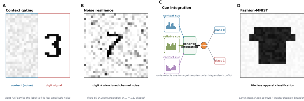
Figure S18: Synthetic benchmark schematics. (A) Context gating: the right half carries the MNIST digit; the left half is filled with low-amplitude uniform noise. (B) Noise resilience: MNIST image corrupted by structured channel noise (fixed 50-D latent projection, \sigma_{\text{task}} = 1.5 , clipped to [0, 1] ). (C) Cue integration: a context cue selects which of two noisy cue streams is reliable; dendritic integration routes the reliable cue to the binary readout. (D) Fashion-MNIST: 10-class apparel classification sharing the MNIST input shape.
