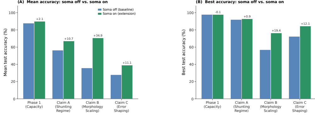
Figure S11: Soma-on extension for LocalCA. Enabling direct somatic input ( somatic_synapses=true ) improves aggregate mean test accuracy across all four paper-facing LocalCA families. Each family is summarized over the completed configs in its matched safeguarded soma-off and soma-on rerun sweeps. The largest gain appears in morphology scaling, where the family mean rises from 35.8% to 70.7% and the best run rises from 57.0% to 76.4%. Gains in the shunting-regime and error-shaping families are smaller but still substantial. Delta labels show soma-on minus soma-off. Because the main mechanistic analysis was developed in the dendrite-only feedforward regime, we report soma-on as a supportive extension rather than replacing the main operating regime.
