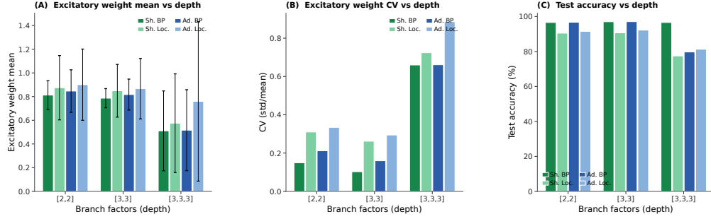
Figure S16: Synaptic weight statistics vs. dendritic depth (MNIST, 5 seeds/cell). (A) Excitatory weight mean (error bars = std). At [2, 2] and [3, 3], all four conditions cluster around 0.8–0.9; at [3, 3, 3] the means drop to \approx 0.5 –0.75 and the cross-seed spread grows, especially for additive LocalCA. (B) Coefficient of variation (CV = std/mean). At shallow/medium depth, LocalCA produces \sim 2\times higher CV than matched BP, but both remain well-behaved ( \leq 0.33 ). At the deepest network all four conditions jump to CV \approx 0.66 –0.88, with additive LocalCA the broadest. (C) MNIST test accuracy. BP tracks \sim 96 –97% at [2, 2]/[3, 3] and \sim 92 –95% at [3, 3, 3]. LocalCA stays within \sim 5 –6 pp of BP at shallow/medium depth but trails by \sim 15 –20 pp at [3, 3, 3], identifying depth as the remaining open challenge for this local rule. The qualitative ordering (shunting LocalCA tracks shunting BP more closely than additive LocalCA tracks additive BP) reinforces the manuscript claim that the conductance denominator is the key mechanistic ingredient.
