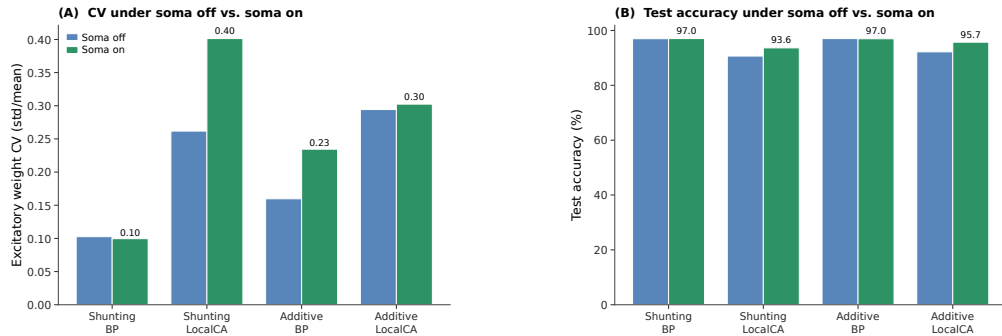
Figure S17: Excitatory-weight CV and MNIST accuracy under soma-off vs. soma-on (depth [3, 3], 5 seeds/cell). (A) Coefficient of variation of excitatory weights for the four (core, strategy) cells; paired bars show soma-off (from Fig. S16) and soma-on (this sweep). Shunting + BP tightens slightly; shunting + LocalCA broadens; additive cells change little. (B) Matched MNIST test accuracy (sanity panel). BP accuracy is preserved or marginally improved; LocalCA accuracy is preserved for additive but drops \sim 3 pp for shunting, consistent with the CV widening in panel A.
