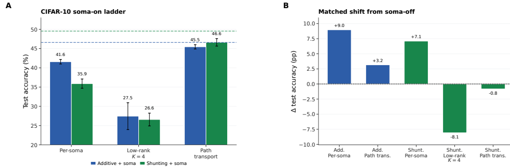
Figure S8: CIFAR-10 compact direct-I-stream depth-4 with somatic_synapses=true . (A) Absolute soma-on ladder on the compact direct-I-stream depth-4 family. Path transport stays strongest in both cores and remains near the matched backprop ceilings (dashed lines), while low-rank K=4 remains weak. (B) Matched shift from soma-off to soma-on for the conditions with a clean paired baseline. Soma helps additive strongly under per-soma and path transport, improves shunting per-soma, leaves shunting transported error close to its soma-off value, and worsens shunting low-rank K=4 . Additive low-rank K=4 is omitted from panel B because the corrected soma-off strong-family mechanism package did not include that exact matched rerun.
