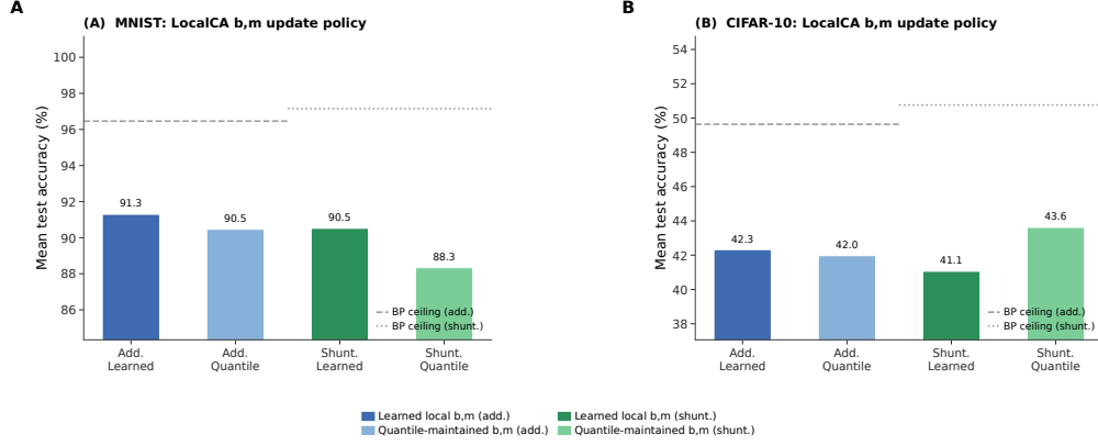
Figure S13: (b, m) update policy under quantile initialization. Each cluster of bars compares the mean test accuracy of learned local (b, m) and quantile-maintained (b, m) under LocalCA for additive and shunting cores, averaged across a matched morphology/init grid [2, 2] and [3, 3, 3] ; analytical and quantile init variants). Dashed and dotted horizontal lines mark the matched standard backpropagation ceiling for additive and shunting respectively. Left (MNIST): Learned local (b, m) is consistently better; quantile-maintained lags by 1.9 pp (additive) and 3.4 pp (shunting) on mean accuracy. Right (CIFAR-10): The gap reverses for shunting; quantile-maintained reaches 43.6% mean vs. 40.3% for learned local, while additive is essentially tied. The pattern suggests that quantile-maintained (b, m) prevents over-fitting the reactivation gate on harder inputs, making it a useful alternative in harder visual regimes.
