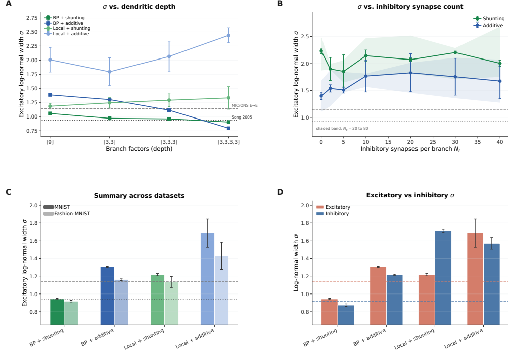
Figure S15: Synaptic weight distribution sensitivity to architecture. (A) Log-normal \sigma vs. dendritic depth (branch factors [9] to [3,3,3,3]). Both backprop and local shunting remain closer to the biological-width references than their additive counterparts across depth. (B) \sigma vs. inhibitory synapses per branch ( N_I ). Without inhibition ( N_I=0 ), all conditions are overly broad; with biologically constrained N_I=10 –20, shunting enters the biological range. Shaded bands show the sweep over N_E=20 to 80. (C) Summary of MNIST and Fashion-MNIST results with biological references. The shunting ordering is consistent across datasets. (D) Excitatory vs. inhibitory weight \sigma on MNIST with MICrONS E→E and I→E reference bands.
