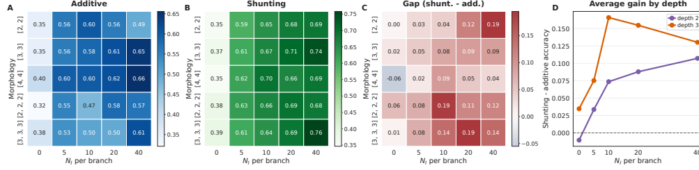
Figure 6: Morphology shifts the inhibitory regime where shunting helps most. (A) Additive LocalCA remains comparatively flat across morphologies and inhibitory synapse counts, with only isolated high-variance pockets. (B) Shunting LocalCA shows a clear morphology-dependent regime: the strongest performance appears at low or moderate inhibition, and the best N_I shifts with tree shape. (C) The shunting-minus-additive gap is largest for wider two-level trees at low inhibition and for deeper trees at modest inhibition, then weakens or vanishes at high inhibition. (D) Averaging by depth highlights the same crossover: depth-2 trees peak near N_I=0 , whereas depth-3 trees retain their largest shunting advantage around N_I=5 .
