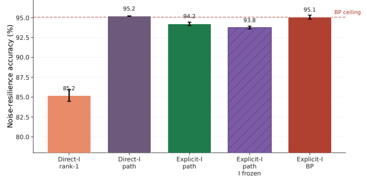
Figure S10: Pathwise inhibition story and one-layer input-mode probe. (A) In a branched conductance tree, the error path gain \alpha_n is the product of local input resistances and dendritic coupling conductances along the path to the soma. Inhibitory conductance on any compartment along that path lowers local input resistance and attenuates all upstream credit paths. (B) The same branch-level inhibitory conductance can be supplied directly from a nonnegative inhibitory input stream (input_mode=1) or through an explicit feedforward inhibitory cell (input_mode=0). (C) The clean mechanism probe keeps the dendritic tree depth ([3,3]) but uses only one feedforward dendritic population; adding a second feedforward E/I layer tests a deeper graph-credit problem rather than the path-gain mechanism itself. (D) Noise-resilience results for the one-layer probe. Direct-I path transport reaches the explicit-I backprop ceiling, and explicit inhibitory cells with path-transport LocalCA also remain near ceiling. This supports the interpretation that explicit inhibitory cells can generate useful path-gain structure when the architecture isolates the dendritic-path question.
