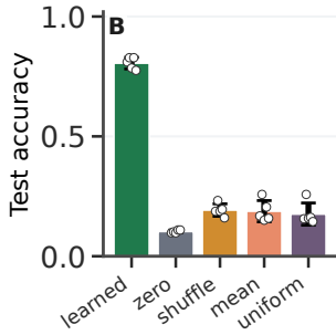
Noise resilience
