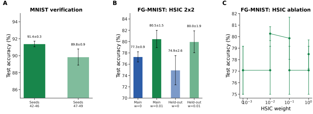
Figure S5: Verification and reproducibility (supplementary). (A) MNIST verification: main seeds (42–46) yield 91.4 \pm 0.3\% ; held-out seeds (47–49) yield 89.8 \pm 0.9\% , showing robustness across random seeds. (B) Matched figure-ground MNIST HSIC control: both main seeds (42–46) and held-out seeds (47–49) compare HSIC weight 0 against 0.01. (C) HSIC weight ablation on figure-ground MNIST: moderate weights (0.01–0.1) perform best.
