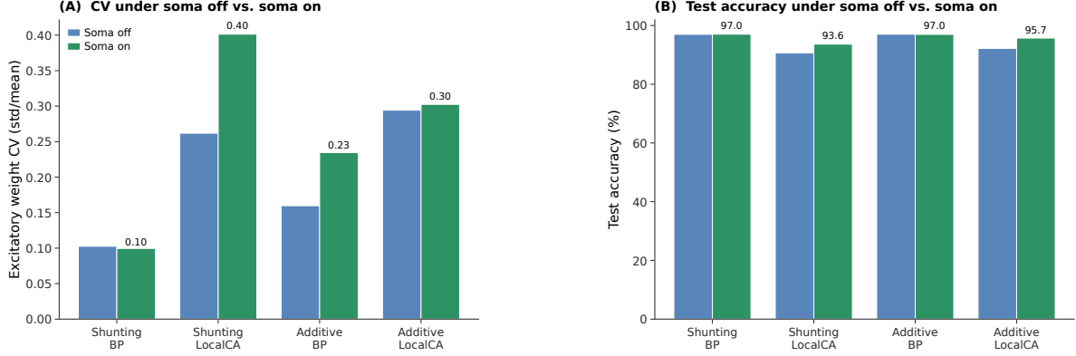
Figure S16: Excitatory-weight CV and MNIST accuracy under soma-off vs. soma-on (depth [3, 3], 5 seeds/cell). (A) Coefficient of variation of excitatory weights for the four (core, strategy) cells; paired bars show soma-off (from Fig. S15) and soma-on (this sweep). Shunting + BP tightens slightly; shunting + LocalCA broadens; additive cells change little. (B) Matched MNIST test accuracy (sanity panel). BP accuracy is preserved or marginally improved; LocalCA accuracy is preserved for additive but drops \sim 3 pp for shunting, consistent with the CV widening in panel A.
