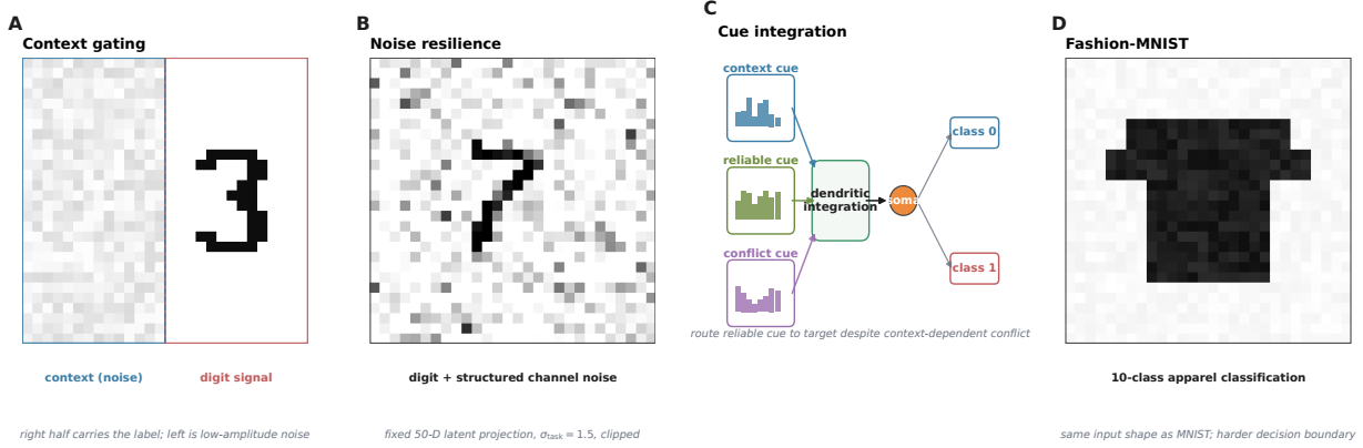
Figure S17: Synthetic benchmark schematics. (A) Context gating: the right half carries the MNIST digit; the left half is filled with low-amplitude uniform noise. (B) Noise resilience: MNIST image corrupted by structured channel noise (fixed 50-D latent projection, \sigma_{\text{task}} = 1.5 , clipped to [0, 1] ). (C) Cue integration: a context cue selects which of two noisy cue streams is reliable; dendritic integration routes the reliable cue to the binary readout. (D) Fashion-MNIST: 10-class apparel classification sharing the MNIST input shape.
