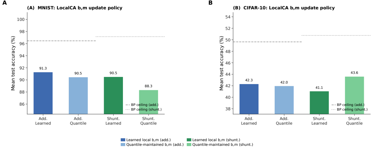
Figure S12: (b, m) update policy under quantile initialization. Each cluster of bars compares the mean test accuracy of learned local (b, m) and quantile-maintained (b, m) under LocalCA for additive and shunting cores, averaged across a matched morphology/init grid ( [2, 2] and [3, 3, 3] ; analytical and quantile init variants). Dashed and dotted horizontal lines mark the matched standard backpropagation ceiling for additive and shunting respectively. Left (MNIST): Learned local (b, m) is consistently better; quantile-maintained lags by 1.9 pp (additive) and 3.4 pp (shunting) on mean accuracy. Right (CIFAR-10): The gap reverses for shunting: quantile-maintained reaches 43.6% mean vs. 40.3% for learned local, while additive is essentially tied. The pattern suggests that quantile-maintained (b, m) prevents over-fitting the reactivation gate on harder inputs, making it a useful alternative in harder visual regimes.
