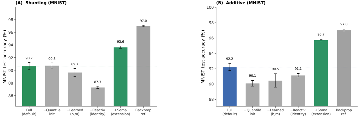
Figure S13: Per-component ablation for LocalCA on MNIST. Bars show mean test accuracy ( \pm s.d. across 5 seeds); coloured bars highlight the manuscript default (blue/green) and the soma-on extension (green). (A) Shunting: The full default reaches 90.7%; removing quantile init leaves accuracy unchanged at 90.8% (quantile init is a mild calibration nudge on this clean task), removing learned ( b, m ) drops by about 1 pp, and removing reactivation entirely drops accuracy to 87.3%; the reactivation transform is the largest single LocalCA ingredient. (B) Additive: Quantile init contributes +2.1 pp (90.1 \rightarrow 92.2%), learned ( b, m ) contributes +1.7 pp, and reactivation contributes +1.1 pp; each ingredient helps on the additive core. Soma-on is the largest positive change in both cores (+3 to +3.5 pp over full config), while matched standard backpropagation reaches 97.0% in both cores and sets the upper reference. The seventh condition (fixed relu reactivation) failed to initialize cleanly under the current quantile path and is omitted.
