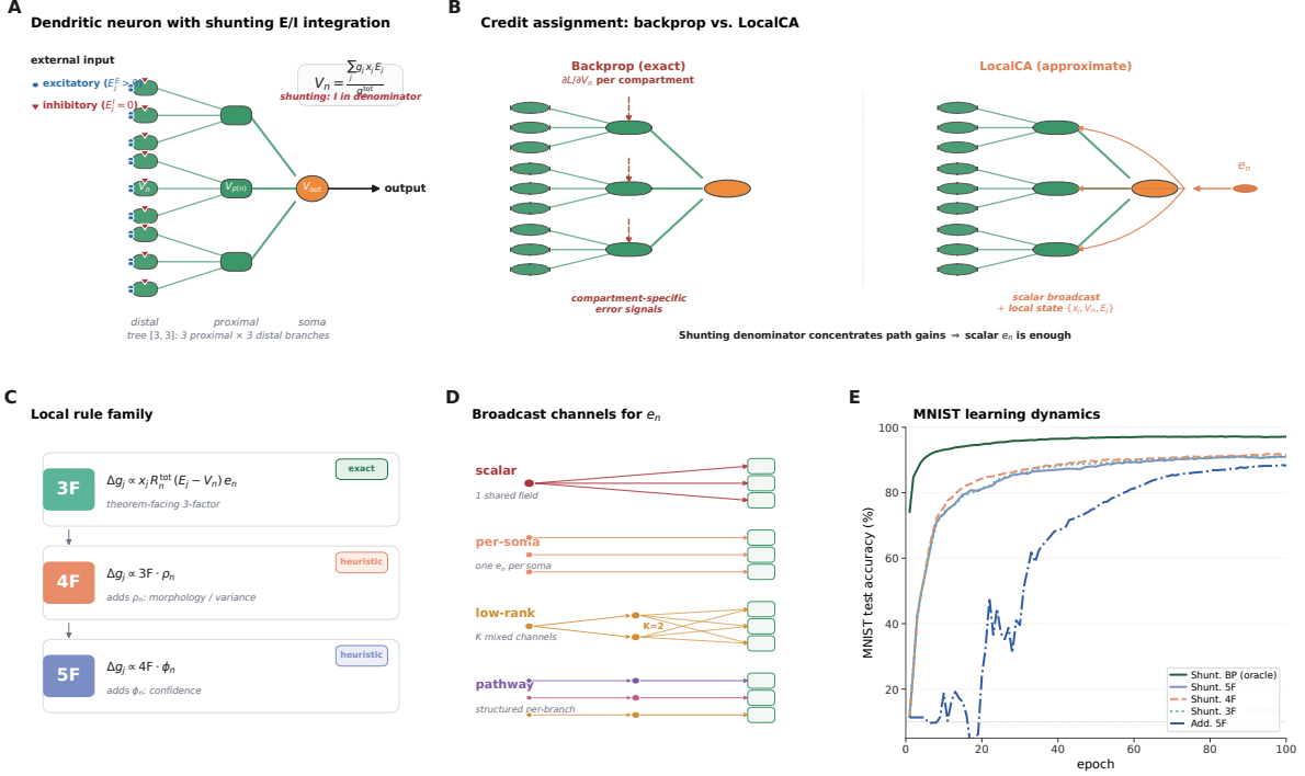
Figure 1: Model and credit assignment. (A) Orientation to the full learning problem. Inputs drive a rooted dendritic tree whose distal compartments feed proximal branches and then the soma. Exact backpropagation supplies compartment-specific errors \partial L / \partial V_n , while LocalCA replaces them with one shared low-bandwidth broadcast e_n ; the synapse update then combines that non-local signal with local quantities available at the compartment. (B) Single-compartment conductance computation. Excitatory synapses, inhibitory synapses, and child branches all contribute to the compartment voltage, while inhibition also enters the total conductance in the denominator. The mini-histograms summarize the visual intuition used throughout the paper: shunting concentrates path gains, whereas additive integration leaves them broad. (C) Local rule family. 3F is the theorem-facing rule; 4F adds the heuristic morphology-aware factor \rho_n ; 5F adds the heuristic confidence-like factor \phi_n . (D) Broadcast approximations. Scalar uses one shared field, per-soma uses a vector when widths match and otherwise falls back to scalar, random low-rank adds a few unstructured channels, and pathway feedback preserves branch identity when different pathways should receive different teaching signals. (E) Representative MNIST learning dynamics from the fixed-epoch Figure 1 sweep. Shunting with the stronger local wrappers tracks backprop much more closely than the additive control, previewing the more quantitative fidelity analyses in Fig. 2.
