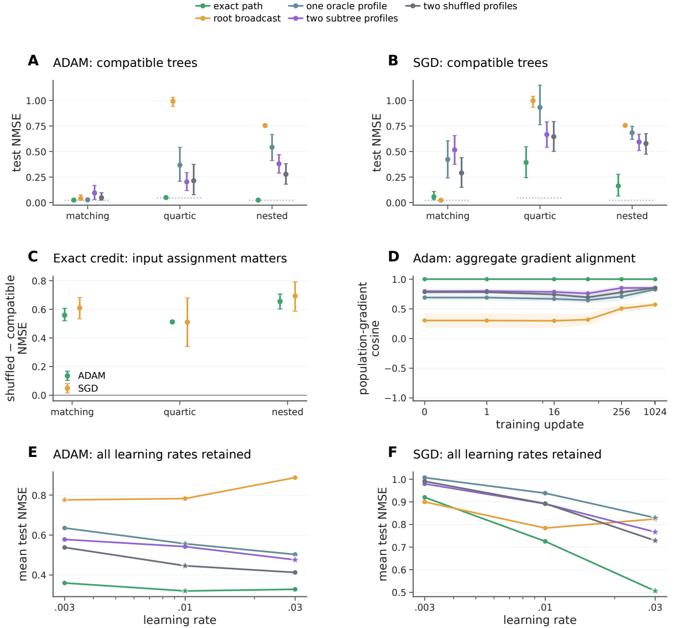
Figure S13: Task-dependent credit requirements in bounded multi-affine trees. A,B, Final test normalized mean squared error (NMSE) on oracle-compatible trees under Adam and stochastic gradient descent (SGD), respectively. Exact path, root broadcast, one oracle profile, two subtree profiles and two shuffled profiles share the forward model, initialization, examples and minibatches. Dotted segments mark known label-noise floors: 0.0225 for matching/nested tasks and 0.045 for quartic tasks. Projection coefficients access the exact current path field and are oracle diagnostics; root broadcast supplies the same scalar error to each internal node. C, Paired exact-credit NMSE increases after shuffling leaf input assignments while preserving tree shape and parameter count. Chance-compatible shuffles are retained. D, Adam gradient cosine between the exact and delivered aggregate clean-population updates, evaluated at each rule's own trained state. Each seed averages the three task families before aggregation; these are not comparisons at a common model state or mean per-example cosines. Points and whiskers in A–C and bands in D are means and pointwise 95% intervals from 10,000 whole-seed bootstrap draws, with twenty independent fresh seeds per family. E,F, Final NMSE at all three learning rates, averaged over both compatible and shuffled assignments and all three families. Stars mark rates selected separately for each rule and optimizer using only development seeds. These means therefore differ from compatible-only panels A,B . Every SGD choice was the upper tested rate; the result is a comparison of the stated training recipes, not a fully optimized SGD limit. Matching and quartic tasks share the input-gradient second moment I_8/4 ; nested tasks have a different spectrum. The oracle-compatible architectures here are independent of the noisy morphology-selection experiment. All 3,600 fresh fits and all tested rates are retained. Panel C is reproduced at the main-text type scale as main Fig. 4H.
