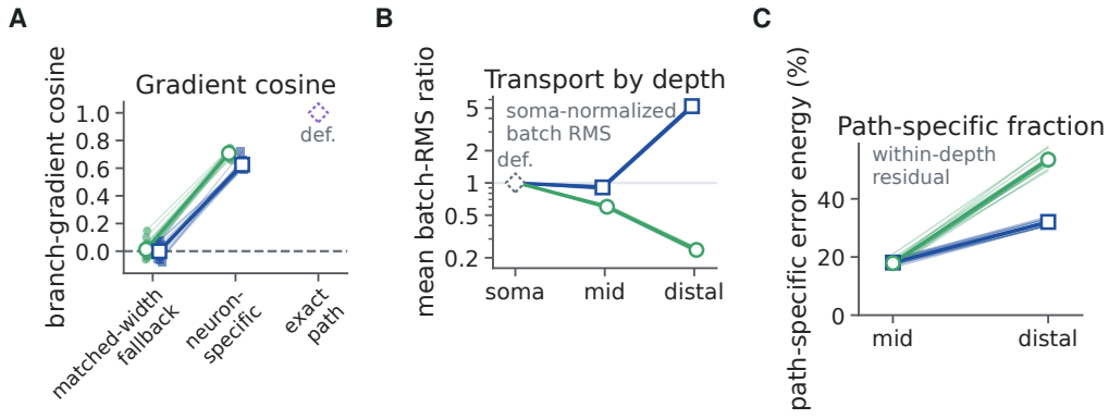
Figure S8: Error-field geometry separates direction, amplitude and spatial variation. Independent fifteen-seed flattened-MNIST cohort of 128 directed [3,3] trees; green circles denote shunting and blue squares raw-additive trees. A , Branch-gradient cosine with the exact gradient at common fixed checkpoints trained with per-neuron feedback; matched-width scalar-fallback and per-neuron fields are evaluated at identical weights and states, and the exact-path cosine of one is definitional. B , Exact voltage-error magnitude by depth at exact-path checkpoints: the batch root-mean-square ratio \text{RMS}(\delta_{n,u}^V) / \text{RMS}(\delta_{0,u}^V) , averaged over neurons and paths, with somatic value one by normalization. C , Within-depth path-specific residual error energy after subtracting the mean across paths within depth d : distal shunting attenuates magnitude but retains the larger path-specific fraction, rising from 18% to 53% (shunting) and 32% (raw additive). Symbols and bars are means and 95% seed-bootstrap intervals. No additional models are trained here; greater path-specific variation did not yield an image accuracy benefit, and voltage- and activation-space capture are different quantities.
