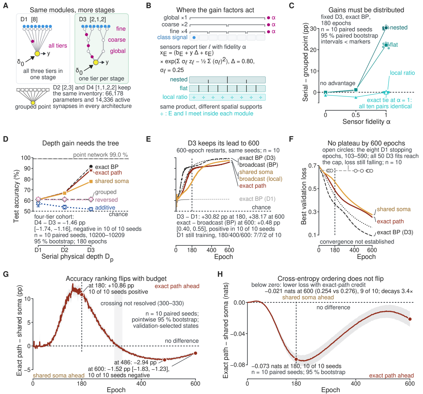
Figure 6: Task organization sets the forward benefit of serial dendrites, and the training budget sets the credit-rule ranking.
