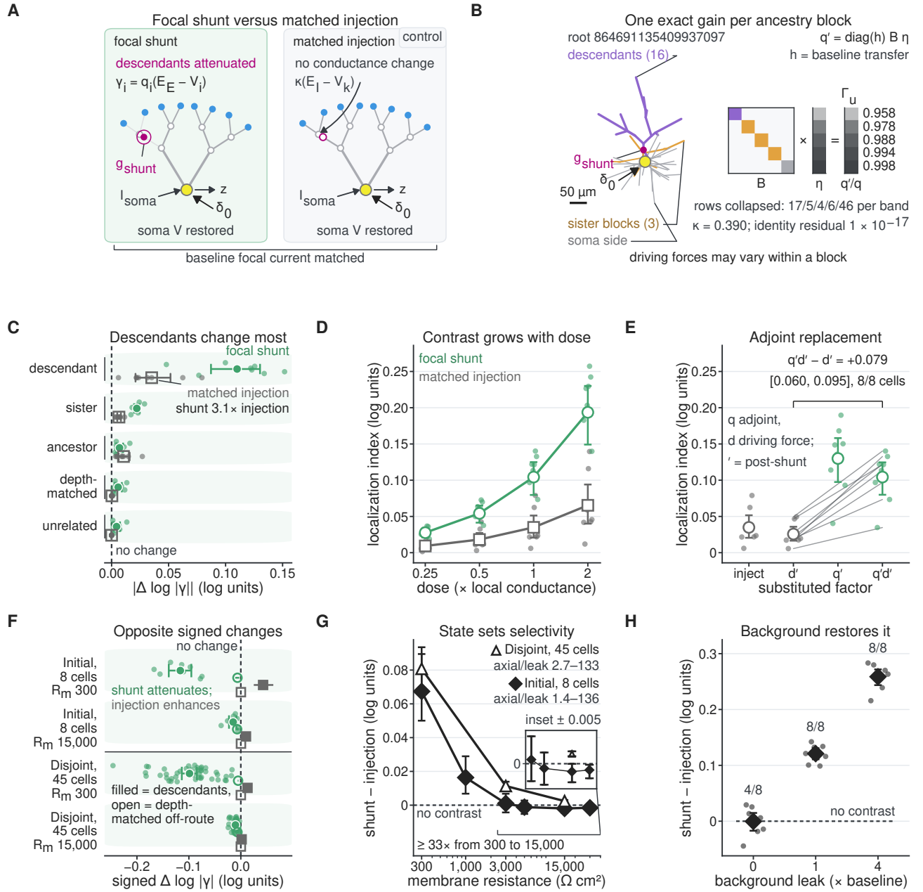
Figure 8: In a passive model, focal shunts apply ancestry-defined gains whose spatial selectivity is set by electrotonic state. A , Two state-matched interventions: a focal inhibitory shunt ( g_{\text{shunt}} , ringed contact; descendants faded) and a matched current injection \kappa(E_I - V_k) (open contact); I_{\text{soma}} restores baseline somatic voltage. Blue, excitatory contacts. Schematic, no data. B , Exact ancestry partition of the median reconstructed cell (as in Fig. 7A) shunted at segment 4227: the site, sixteen descendants, three sister blocks, soma side. Block indicators times one gain per block ( \eta = 0.958\text{--}0.998 , \kappa = 0.390 ) give the adjoint ratio exactly: a physical instance of \Gamma_u (Eq. 4). Scale bar, 50 \mu\text{m} . Anatomical schematic; block sizes and gains are derived (Source Data). C , Absolute log change in gradient magnitude by relation to the site; unit dose, permissive normalized passive parameters; off-route injection changes are at most 3 \times 10^{-4} , zero for unrelated sites by construction. D , The same index against dose normalized to local leak plus synaptic conductance. E , Factor substitution in the exact gradient: injection, driving force ( d' ), adjoint ( q' ), both ( q'd' ). Green, conditions carrying the post-shunt adjoint q' ; grey, the baseline adjoint q . Thin grey lines join the same cell across d' and q'd' ; the bracket is their paired difference. Adding the post-shunt adjoint on top of the substituted driving force ( q'd' - d' ) adds 0.079 log units [0.060, 0.095]. F , Signed log change at two membrane resistances; green circles, focal shunt (attenuates); grey squares, matched current injection (enhances); filled, descendants; open, depth-matched off-route sites. G , Shunt-minus-injection localization against membrane resistance; filled diamonds, initial eight-cell cohort; open triangles, disjoint 45-cell calibration cohort. Inset, the bracketed window: opposite cohort signs at R_m = 15,000 . H , Distributed background conductance restores that contrast at R_m = 15,000 \Omega \text{ cm}^2 , input-conductance-normalized dose one. C–H , unit, a reconstructed cell (sites averaged within cell); symbols and whiskers, cohort means and 95% cell-bootstrap intervals; dots, cells ( F , shunt-descendant series only; omitted in G ); endpoint, the post-intervention steady state, somatic voltage restored. Fill is panel-local and keyed in each panel; in C and E it repeats colour. n = 8 cells (101 focal sites), initial eight-cell cohort, one MICrONS mouse; F and G add the disjoint 45-cell calibration cohort (235 sites). Source Data: source_data/curated_publication/figure_08_plotted.csv.
