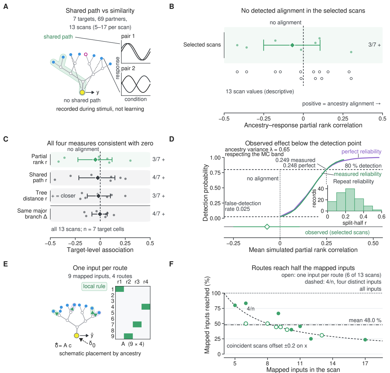
Figure 9: Recorded partner responses show no dendritic-ancestry alignment, and this sample detects only effects above a partial rank correlation of about 0.25. A , The statistic: two contact pairs on one arbor, one sharing a soma-to-ancestor path (green patch), the other linked to the soma by dashed hairlines; filled blue discs, excitatory contacts; open magenta ring, an inhibitory partner; insets, their response comparison. No data; no \delta_0 , these are stimulus recordings. B , Ancestry–response partial rank correlation, selected-scan cohort; dots, the seven target values; open circles, the thirteen all-eligible-scan values (same seven targets, stacked where they coincide); diamond, mean with 95% target-bootstrap interval ( n = 7 target cells): -0.069 [-0.251, 0.106] . C , Same inference, four topology measures, all thirteen scans; means and 95% target-bootstrap intervals ( n = 7 target cells). Top row, the all-eligible-scan partial rank correlation, -0.048 [-0.224, 0.118] . Tree distance is sign-flipped, so positive means closer. Below the rule, same-major-branch \Delta is a difference in mean similarity, not a correlation: its narrower interval reflects smaller units, not greater precision. D , Detection probability against the frozen model’s mean simulated partial rank correlation; shaded 95% Wilson Monte Carlo intervals (half-width \leq 0.016 , narrower than the stroke); the intercept is the false-detection rate, 0.025. The rug locates the observed estimate ( n = 7 target cells, 95% target bootstrap), not a power estimate. Inset, split-half repeat reliability, 123 of 125 partner–scan records (102 partners), the two with negative r omitted. E , Representative scan (median mapped-input count, no outcome selection): nine mapped inputs placed by ancestry beside the realized 9 \times 4 support, with \hat{\delta} = A c imposed, not observed (schematic; dashed \delta_0 ). Route-capsule tints aid separability only; the local rule badge applies to the whole card. Neither encodes a per-route property. F , Mapped inputs reached per scan; open, the six scans whose four routes each reached one input; dashed, 4/n, coverage when four routes reach four distinct inputs. Not a ceiling: two scans fall below (repeated inputs), three above (multi-input routes). Coincident scans are offset \pm 0.2 horizontally; n = 13 scans from seven target cells, descriptive, no interval. No measured positive control exists. Source Data: source_data/curated_publication/figure_09_plotted.csv , source_data/functional_topology_all_scans/ and source_data/credit_first_figures/figure_08_sources.json .
