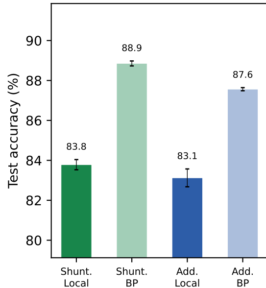
Fashion-MNIST control
