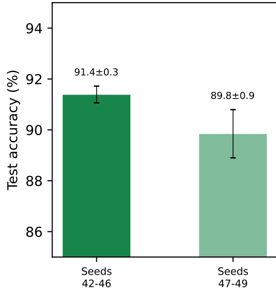
MNIST verification
