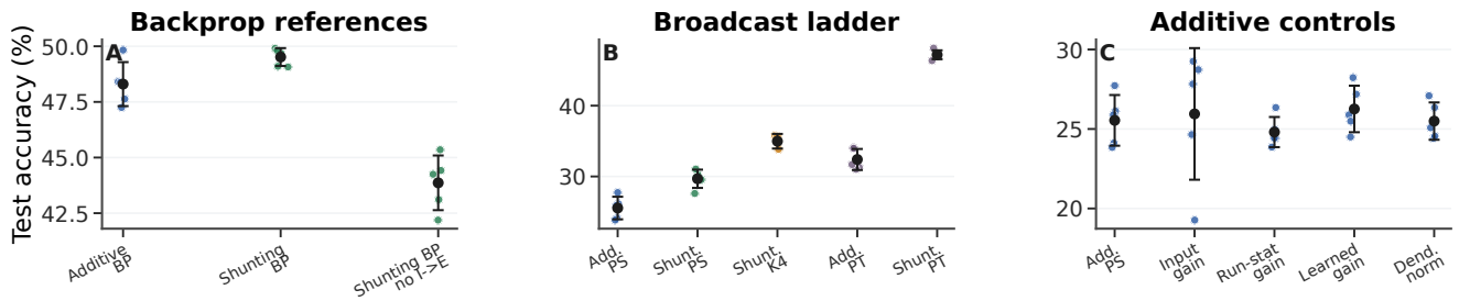
Figure S8: CIFAR-10 control ladder in the compact direct-I-stream family. (A) Matched backprop ceilings. With nonnegative inputs and a nonlinear decoder, shunting slightly exceeds additive under standard training, and removing learned I-to-E conductance lowers the shunting ceiling. (B) Broadcast ladder. Per-soma feedback remains weak on this harder dataset, random low-rank K=4 improves partially, and exact effective transported error nearly reaches the shunting backprop ceiling. (C) Additive fairness controls. Input-dependent gain, running-stat gain, learned gain, and dendritic normalization do not rescue additive per-soma feedback. This figure is a harder-dataset stress test, not a claim of competitive CIFAR-10 benchmarking.
