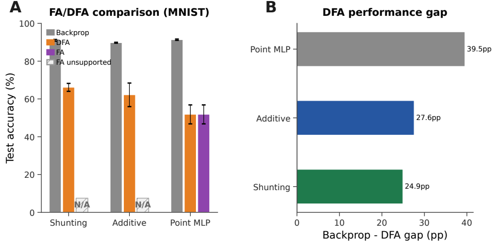
Figure S6: Feedback alignment baselines (MNIST) . (A) Grouped comparison: standard backprop (neutral gray), DFA (orange), and FA (purple). Hatched N/A markers indicate that FA is not implemented for the block-structured dendritic architectures because the random feedback matrices are not dimensionally compatible with the tree-structured branch updates. DFA achieves 66.1% on shunting vs. 62.2% additive vs. 51.8% point MLP. (B) Backprop–DFA gap: dendritic architectures (24.9–27.6 pp) show smaller gaps than point MLPs (39.5 pp), suggesting conductance-based architecture is partially compatible with random feedback.
