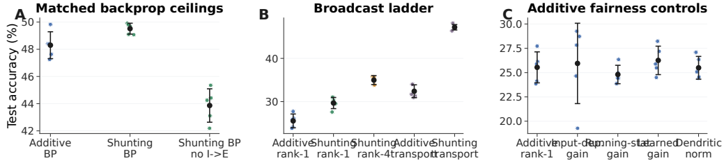
Figure S7: CIFAR-10 control ladder in the compact direct-I-stream family . (A) Matched backprop ceilings. With nonnegative inputs and a nonlinear decoder, shunting slightly exceeds additive under standard training, and removing learned I-to-E conductance lowers the shunting ceiling. (B) Broadcast ladder. Rank-1 broadcast remains weak on this harder dataset, rank-4 improves partially, and exact effective transported error nearly reaches the shunting backprop ceiling. (C) Additive fairness controls. Input-dependent gain, running-stat gain, learned gain, and dendritic normalization do not rescue additive rank-1 broadcast. This figure is a harder-data diagnostic, not a claim of competitive CIFAR-10 benchmarking.
