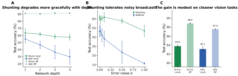
Figure S5: Additional stress tests. (A) Depth scaling: shunting local (green) degrades more gracefully from 63.5\% to 57.4\% ; additive local (blue) drops from 54.9\% to 29.7\% . Backprop ceilings (dashed) remain stable. (B) Broadcast-noise robustness: shunting remains stable for \sigma \leq 0.1 ; additive degrades rapidly and reaches chance at \sigma = 1 . (C) Fashion-MNIST: the shunting gain is modest on this cleaner benchmark ( 83.8\% local vs. 88.9\% backprop), consistent with the regime-dependent story in the main text.
