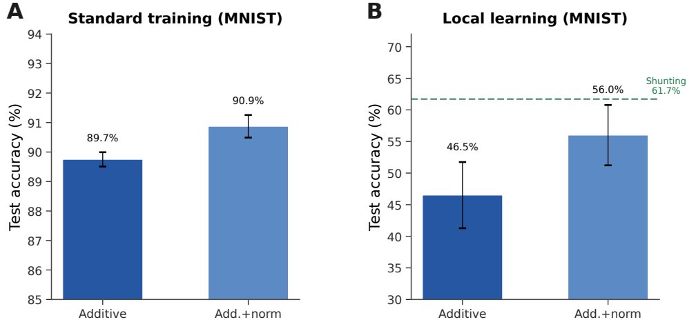
Figure S8: Additive + normalization control (MNIST stress-regime diagnostic). (A) Standard backprop: normalization provides a small boost (89.7% → 90.9%). (B) Local learning: normalization improves additive from 46.5% to 56.0% (+9.5 pp), partially closing the gap to shunting (61.7%, dashed green). These lower local accuracies come from a separate stress-regime diagnostic, not from the capacity-calibrated competence setting in Table S2.
