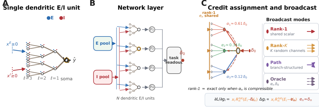
Figure 1: Model and credit assignment. (A) Single dendritic E/I unit: nonnegative excitatory and inhibitory input streams drive a 3-level branched tree of conductance compartments; each branch carries E and I synapses; the gold-ringed soma matches the highlighted unit in B. (B) Network layer: E and I input pools feed N dendritic E/I units; per-unit somas project to a task readout, and \delta_0 = \partial L / \partial V_0 is the somatic error available for broadcast. (C) Credit assignment and broadcast taxonomy: exact credit varies by path through the conductance-stage path gains \alpha_n \delta_0 , whereas rank-1 LocalCA shares one error field across compartments; the four broadcast modes used in the paper (Rank-1, Rank- K , Path, Oracle) trade bandwidth for fidelity. The local eligibility (orange) and broadcast factor (red) factorize the gradient as shown in the bottom equation strip.
