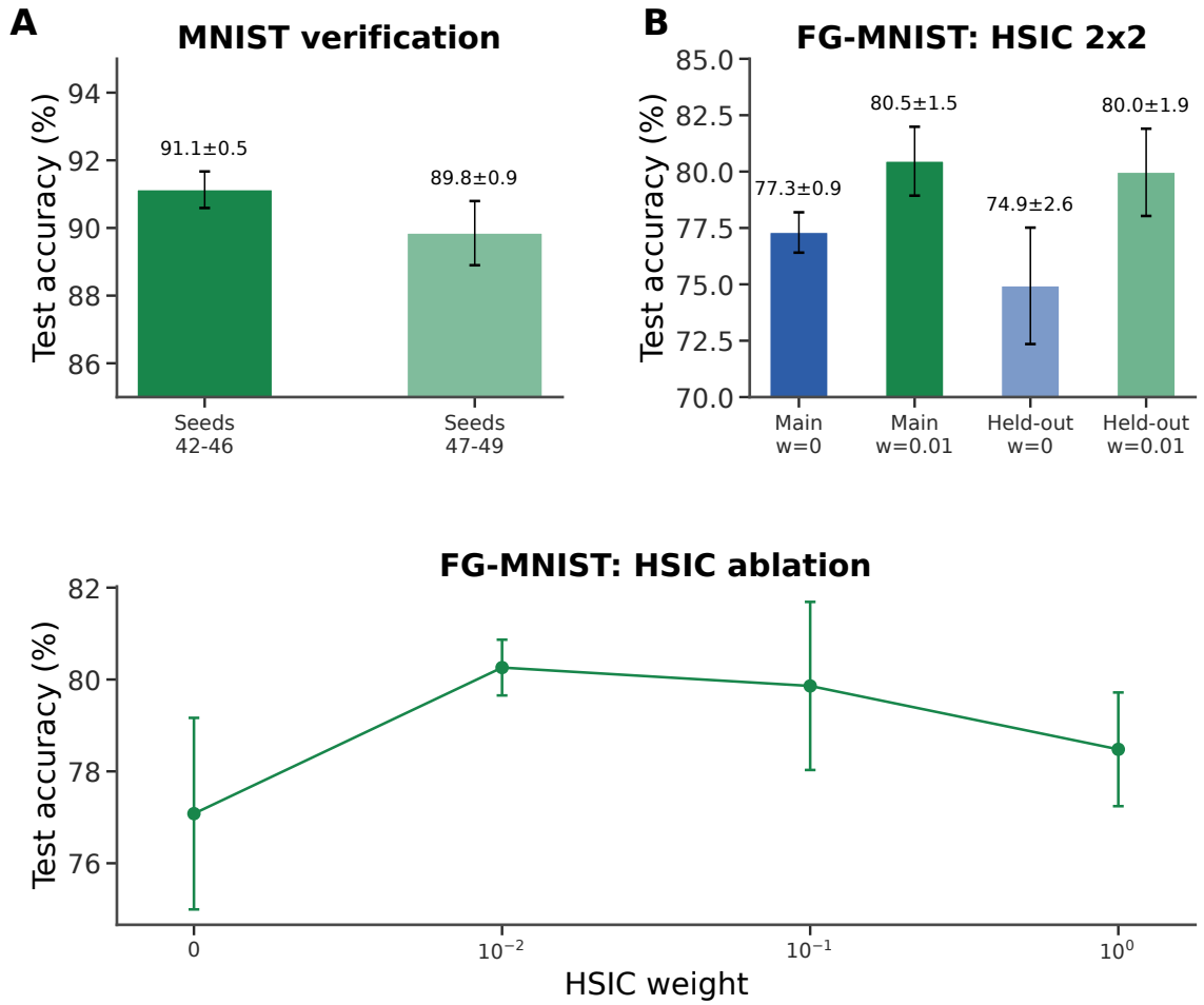
Figure S5: Verification and seed robustness (supplementary). (A) MNIST verification: repeat runs on main seeds (42–46) yield 91.1 \pm 0.5\% ; held-out seeds (47–49) yield 89.8 \pm 0.9\% , showing robustness across random seeds. (B) Matched figure-ground MNIST HSIC control: both main seeds (42–46) and held-out seeds (47–49) compare HSIC weight 0 against 0.01. (C) HSIC weight ablation on figure-ground MNIST: moderate weights (0.01–0.1) perform best.
