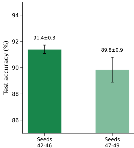
MNIST verification
