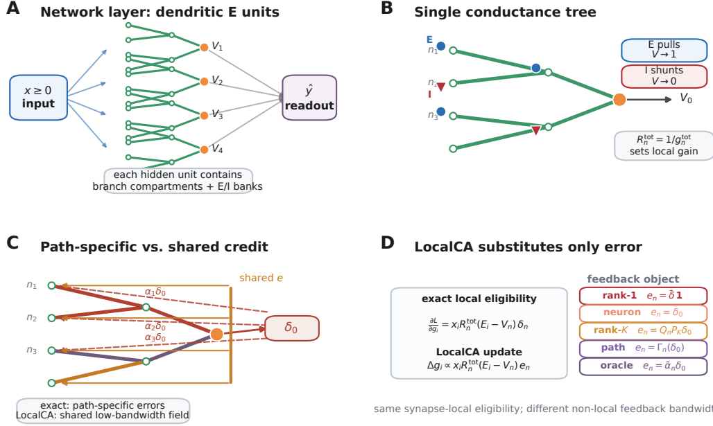
Figure 1: Model and credit assignment. (A) Network layer in which each hidden excitatory unit is a dendritic conductance tree. (B) Single dendritic unit with nonnegative excitatory drive, inhibitory shunting load, and input-resistance-dependent gain. (C) Exact compartment errors are path-specific transports of the somatic error, whereas rank-1 LocalCA sends one shared field from the same somatic side. (D) LocalCA keeps the exact synapse-local eligibility and substitutes e_n \approx \delta_n ; rank-1, neuron-wise, rank- K , path-structured, and transported-oracle feedback trade bandwidth for fidelity.
