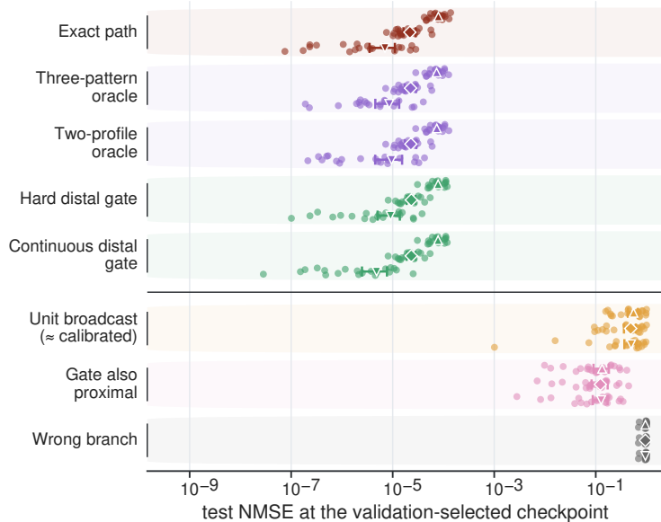
Opposed task, 4,096 updates
