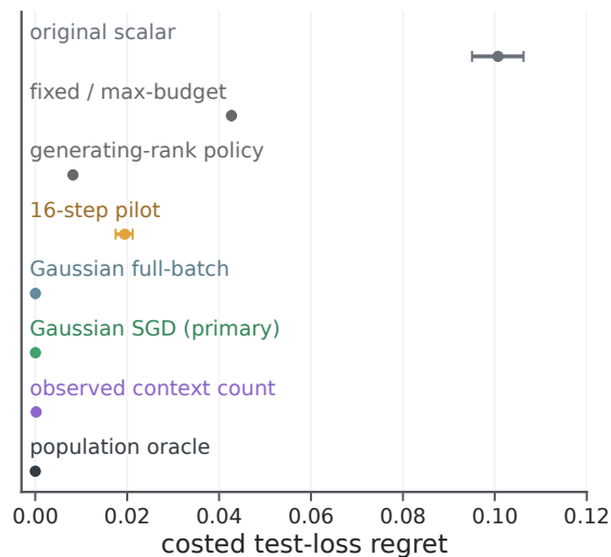
Joint transfer: final selection
