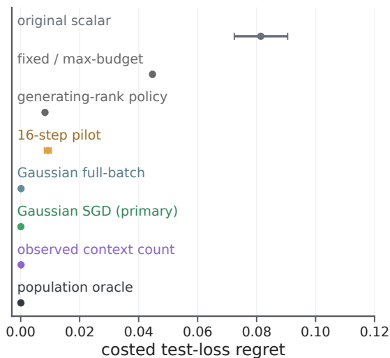
Feedback only: final selection
