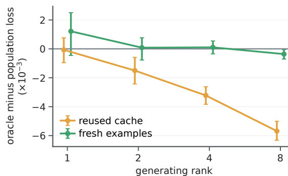
Joint transfer: cache sensitivity
