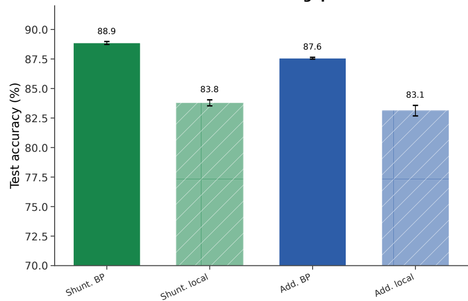
Fashion-MNIST gap
