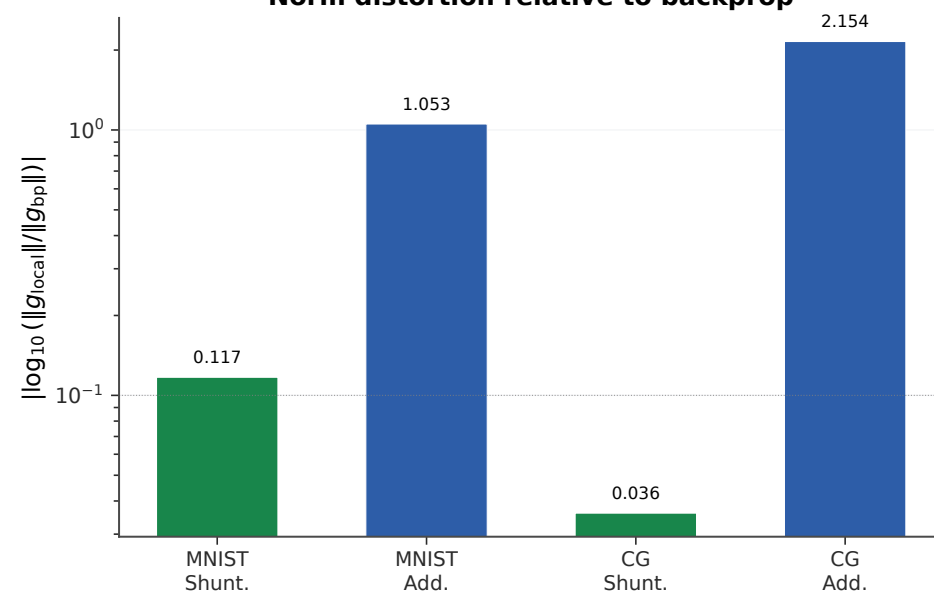
Norm distortion relative to backprop
