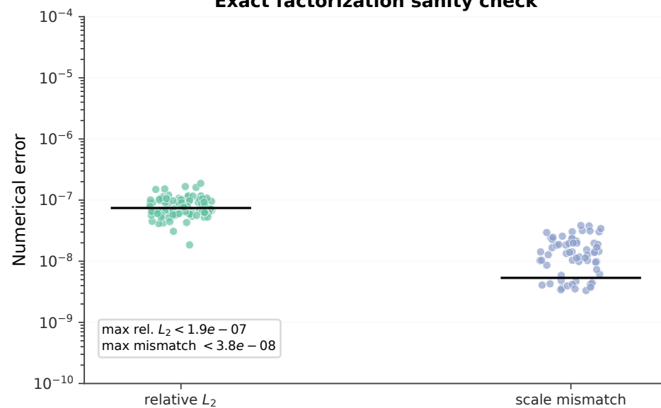
Exact factorization sanity check
