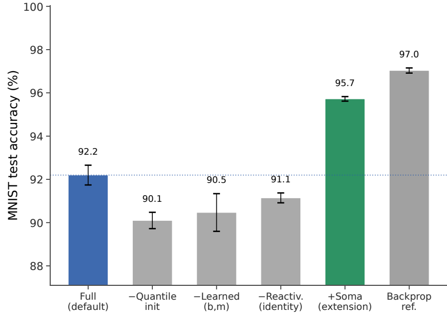
(B) Additive (MNIST)
