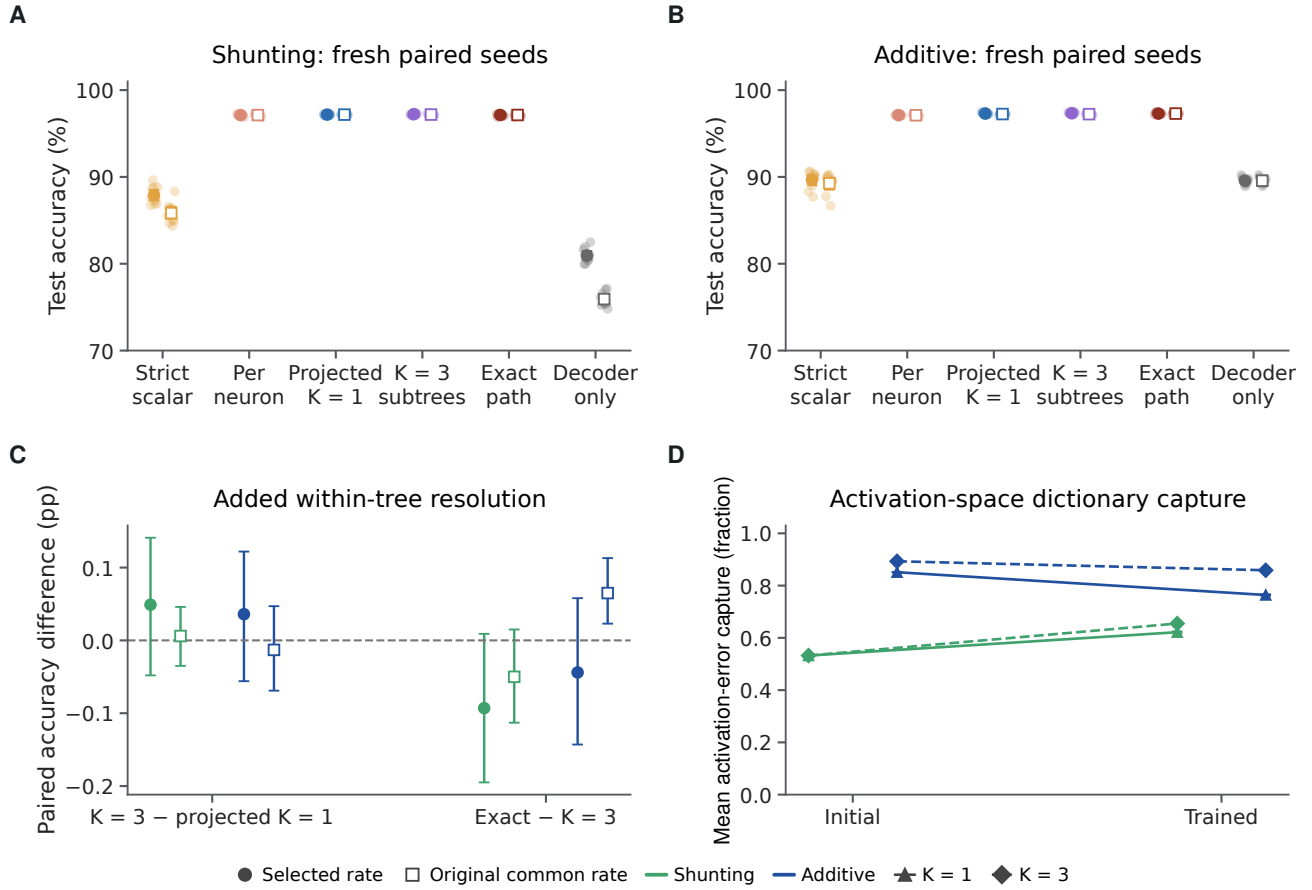
Figure S7: Intermediate dictionaries capture more image-task credit without improving accuracy. A,B , Six-rule MNIST ladder in shunting and raw-additive networks; ten fresh paired seeds per architecture. Filled/open symbols use development-selected/original common rates. In A and B colour names the rule at each tick (amber, strict scalar; salmon, per neuron; blue, projected K = 1 ; violet, K = 3 subtrees; dark red, exact path; grey, decoder only); in C and D colour names the architecture (green, shunting; blue, raw additive). Where the selected multiplier equals the original common rate (shunting per neuron, projected K = 1 and exact path; additive exact path and decoder only) the filled and open symbols are the same ten runs drawn twice. The four dendritic arms lie within 0.25 percentage points of one another in each architecture, below the symbol size at this scale; their paired within-tree contrasts are resolved in C . Decoder-only learning freezes the initialized core. C , Paired accuracy differences for three profiles versus a projected common profile, and exact versus three-profile credit; filled and open as in A,B . Note the scale: the full y range of C is 0.35 percentage points, about one eightieth of the 30-point range of A and B . The number of seeds (of ten) with a positive difference is 7, 5, 5 and 3 for the four K = 3 minus projected K = 1 marks and 3, 4, 4 and 7 for the four exact minus K = 3 marks, in the order drawn (shunting selected, shunting common, additive selected, additive common). D , Initial and trained mean activation-error capture (fraction) by uniform K = 1 (triangles, solid lines) or subtree K = 3 (diamonds, dashed lines) profiles, averaged over 2,048 held-out images within each seed; at shunting initialization the two profiles coincide (0.532 for both) and the triangle lies under the diamond. Projection coefficients use the exact activation-error field of this ten-seed cohort, so D reproduces the K = 1 and K = 3 points of main Fig. 1G for this cohort; voltage-space capture and the aggregate energy capture of the same fits are retained in Source Data and are not the plotted quantity. A and B show the ten per-seed values with the mean and no interval bars; C draws means with descriptive 95% seed-bootstrap intervals; the intervals in D are at most 0.007 capture units, below the symbol size, and are not drawn. Greater capture did not yield an image accuracy benefit. All image cohorts have one dendritic layer and a linear readout.
