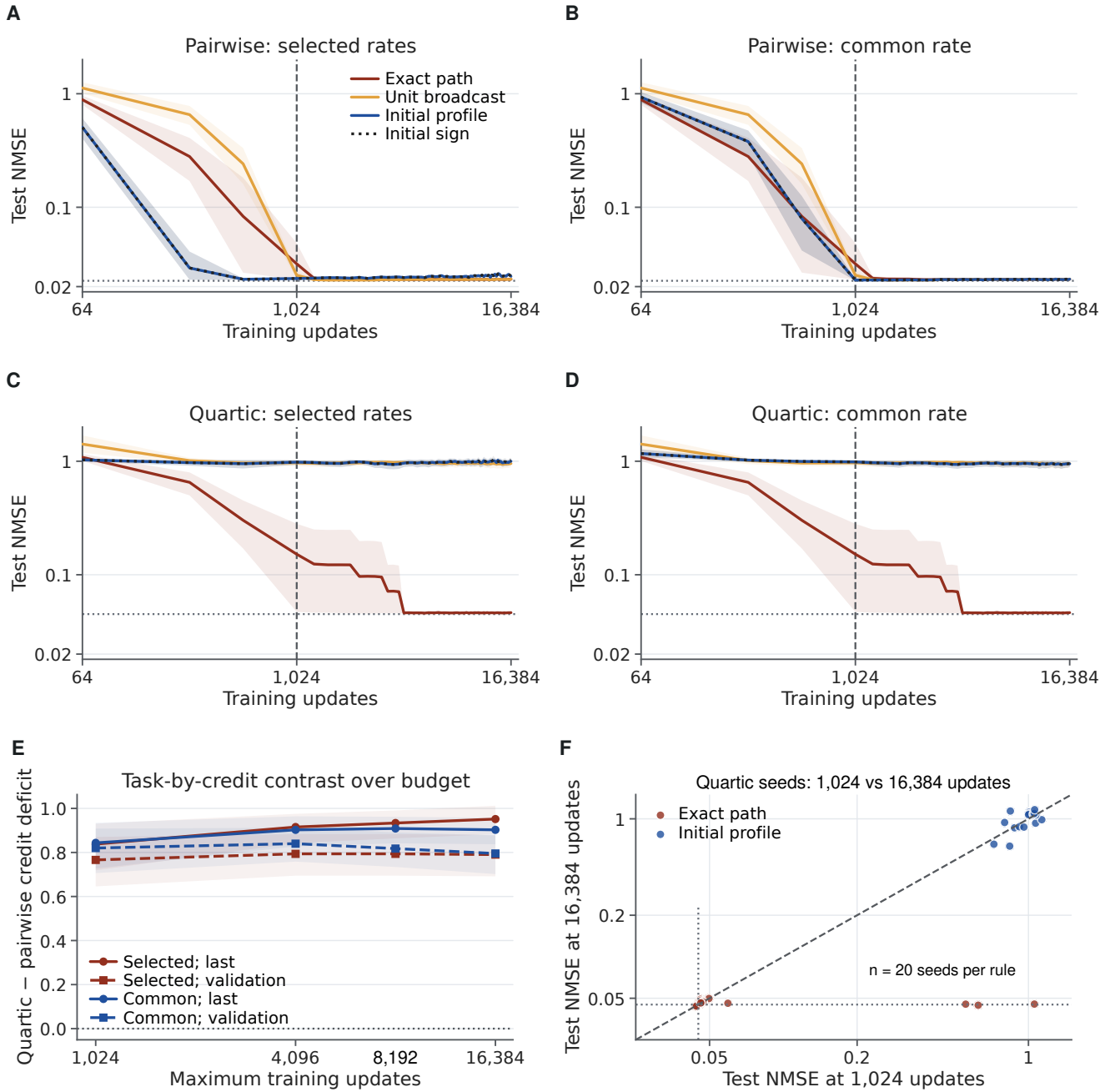
Figure S16: Longer matched budgets retain the task-dependent fixed-profile deficit. A,B , Pairwise targets under Adam at the separately selected rates and at the common rate (0.003), with exact, unit-broadcast, initial-profile and initial-sign credit; initial profile is the calibrated-broadcast rule of main Fig. 4 and initial sign keeps only its signs. In A–D and F colour names the credit rule: dark red, exact path; amber, unit broadcast; blue, initial profile; black dotted, initial sign. C,D , Quartic targets at the same two rate choices. Dashed verticals mark 1,024 updates; dotted horizontals the noise-only NMSE (0.0225 pairwise, 0.045 quartic). Drawn checkpoints are 64, 256, 512, 1,024 and every 256 updates thereafter; curves are straight segments between them. Exact and unit-broadcast selected rates equal the common rate, so those curves are the same runs in A,B and in C,D ; initial sign traces initial profile in A, B and D (within 0.03 in C ) because positive profile scaling largely cancels in Adam. At 16,384 updates the pairwise means are 0.0232 (exact), 0.0233 (unit) and 0.0247 (profile and sign) in A and 0.0232, 0.0233 and 0.0233 in B , within the line width. E , Quartic-minus-pairwise difference in initial-profile-minus-exact NMSE at budgets 1,024, 4,096, 8,192 and 16,384: circles/solid, terminal states; squares/dashed, validation-selected states. Here colour names the rate view, not the credit rule: dark red, rates selected per rule (the series of main Fig. 4F); blue, the common rate. The dotted line marks zero; the four 95% bands overlap heavily, together spanning 0.65–1.01. F , All twenty exact-path and twenty initial-profile quartic seeds at 1,024 and 16,384 updates; the dashed diagonal marks unchanged error, the dotted guides the quartic noise-only NMSE; sixteen exact seeds lie within 0.044–0.050 on both axes and overplot. F resolves the three stalled seeds of main Fig. 4D; A and C repeat the selected-rate curves of main Fig. 4C,D. Curves show means and descriptive 95% whole-seed bootstrap intervals. All 720 trajectories (twenty seed blocks, three tasks, four rules, two optimizers, both rate choices) are retained and the original endpoints replay exactly. Rates remain fixed and coefficients bounded; this is a retrospective-cohort extension under a prospective protocol, not fresh confirmation.
