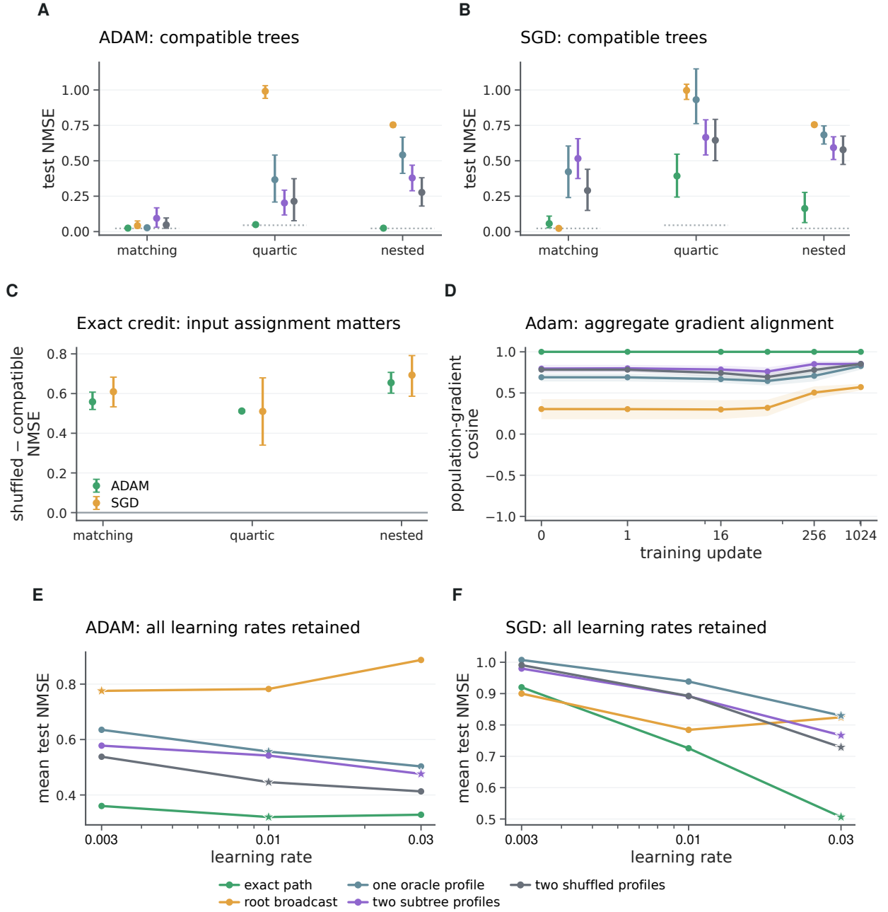
Figure S13: Task-dependent credit requirements in bounded multi-affine trees. A,B , Final test normalized mean squared error (NMSE) on oracle-compatible trees under Adam and stochastic gradient descent (SGD), respectively. Exact path (green), root broadcast (amber), one oracle profile (slate blue), two subtree profiles (violet) and two shuffled profiles (dark grey) share the forward model, initialization, examples and minibatches; this key is specific to this figure (exact path is red-brown in the main figures). Dotted segments mark known label-noise floors: 0.0225 for matching/nested tasks and 0.045 for quartic tasks. Projection coefficients access the exact current path field and are oracle diagnostics; root broadcast supplies the same scalar error to each internal node. C , Paired exact-credit NMSE increases after shuffling leaf input assignments (not the shuffled-profiles rule) while preserving tree shape and parameter count; green and amber here mean Adam and SGD, both under exact credit, and the Adam quartic interval (0.507–0.517) is hidden by its marker. D , Adam gradient cosine on oracle-compatible trees between the exact and delivered aggregate clean-population updates, evaluated at each rule’s own trained state after 0, 1, 16, 64, 256 and 1,024 updates (0 drawn left of the log axis); the exact-path cosine is 1 by definition. Each seed averages the three task families before aggregation; these are not common-state or mean per-example cosines. Points and whiskers in A–C and bands in D are means and pointwise 95% intervals from 10,000 whole-seed bootstrap draws, twenty fresh seeds per family. E,F , Final NMSE at learning rates 0.003, 0.01 and 0.03, averaged over both compatible and shuffled assignments and all three families; points are means over the same twenty seeds, without intervals, on different NMSE axes in E and F . Stars mark rates selected separately for each rule and optimizer using only development seeds. Matching and quartic tasks share the input-gradient second moment I_8/4 ; nested tasks have a different spectrum. The Adam series of C is the contrast of main Fig. 4H (drawn there horizontally with the paired seeds and a pooled row; “matching” is “Pairwise” there); C adds the SGD arm.
