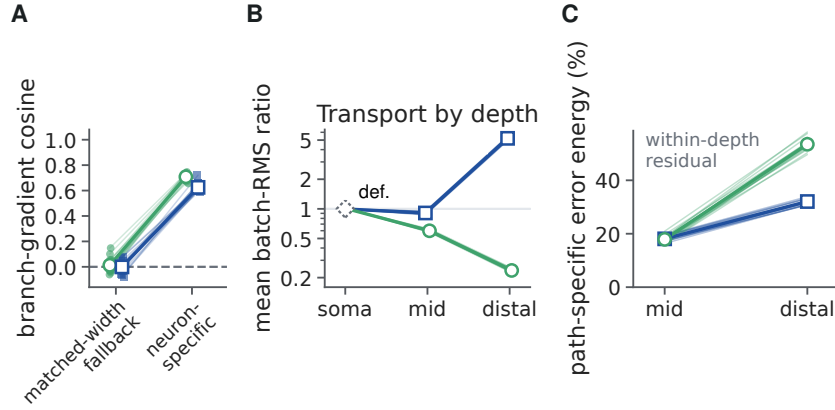
Figure S8: Error-field geometry separates direction, amplitude and spatial variation. Independent fifteen-seed flattened-MNIST cohort of 128 directed [3, 3] trees; green circles denote shunting and blue squares raw-additive trees. A , Branch-gradient cosine with the exact gradient at common fixed checkpoints trained with per-neuron feedback; matched-width scalar-fallback and per-neuron fields are evaluated at identical weights and states, and the exact-path cosine is one by construction and is not drawn. B , Exact voltage-error magnitude by depth at exact-path checkpoints: the batch root-mean-square ratio \text{RMS}(\delta_{n,u}^V)/\text{RMS}(\delta_{0,u}^V) , averaged over neurons and paths, with somatic value one by normalization; the open dashed diamond at soma (def.) marks this normalization constant, not a measurement. C , Within-depth path-specific residual error energy after subtracting the mean across paths within depth d : distal shunting attenuates magnitude but retains the larger path-specific fraction, rising from 17.9% (shunting) and 18.1% (raw additive), where the two mid symbols overlap, to 53% and 32%. Thin lines in A and C are the fifteen individual seeds per architecture and symbols are seed means; B draws seed means only. The 95% seed-bootstrap intervals are drawn as bars but are hidden by the symbols (half-widths at most 0.03 in A , 0.08 in B and 1.2 percentage points in C ). No additional models are trained here; greater path-specific variation did not yield an image accuracy benefit, and voltage- and activation-space capture are different quantities.
