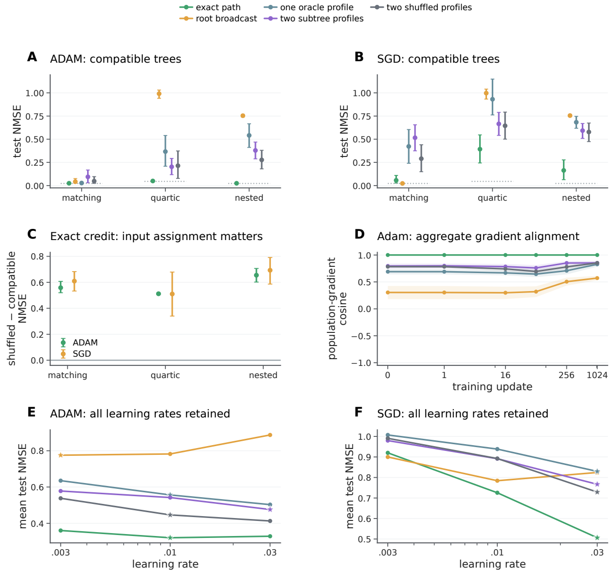
Figure S12: Task-dependent credit requirements in bounded multi-affine trees. A,B, Final test normalized mean squared error (NMSE) on oracle-compatible trees under Adam and stochastic gradient descent (SGD), respectively. Exact path, root broadcast, one oracle profile, two subtree profiles and two shuffled profiles share the forward model, initialization, examples and minibatches. Dotted segments mark known label-noise floors: 0.0225 for matching/nested tasks and 0.045 for quartic tasks. Projection coefficients access the exact current path field and are oracle diagnostics; root broadcast supplies the same scalar error to each internal node. C, Paired exact-credit NMSE increases after shuffling leaf input assignments while preserving tree shape and parameter count. Chance-compatible shuffles are retained. D, Adam gradient cosine between the exact and delivered aggregate clean-population updates, evaluated at each rule's own trained state. Each seed averages the three task families before aggregation; these are not comparisons at a common model state or mean per-example cosines. Points and whiskers in A–C and bands in D are means and pointwise 95% intervals from 10,000 whole-seed bootstrap draws, with twenty independent fresh seeds per family. E,F, Final NMSE at all three learning rates, averaged over both compatible and shuffled assignments and all three families. Stars mark rates selected separately for each rule and optimizer using only development seeds. These means therefore differ from compatible-only panels A,B . Every SGD choice was the upper tested rate; the result is a comparison of the stated training recipes, not a fully optimized SGD limit. Matching and quartic tasks share the input-gradient second moment I_8/4 ; nested tasks have a different spectrum. The oracle-compatible architectures here are independent of the noisy morphology-selection experiment. All 3,600 fresh fits and all tested rates are retained.
