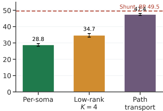
B Shunting rank bridge
