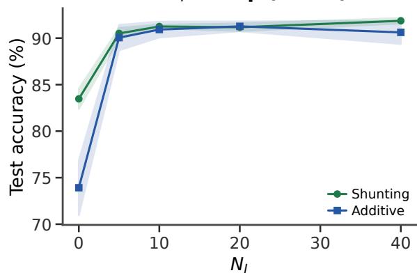
C MNIST N_I sweep (detail)
