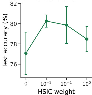
C HSIC ablation
