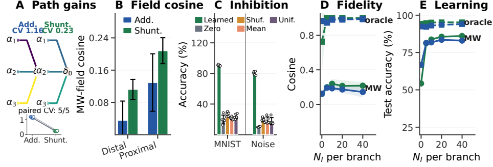
Figure 3: Mechanistic chain from path gains to learning. (A) Conductance-stage path-gain field \alpha^{\text{cond}} at N_I=5 ; the inset shows the five paired-seed CV values, with lower shunting CV in every pair. (B) Stage-resolved cosine between the submitted matched-width/scalar-fallback field and the exact MNIST error on distal and proximal compartments, averaged over train, validation, and test batches within each of five checkpoints. The width-matched somatic stage is excluded because its cosine is one by construction in both cores. Fidelity is low on both dendritic stages, and the five-checkpoint comparison is descriptive rather than evidence for a cross-core ordering. (C) Post-training inhibitory-conductance interventions. (D,E) Fidelity and learning with matched-width/scalar-fallback feedback (MW) or exact transported error (oracle) on noise resilience. CV denotes the coefficient of variation over the sampled path-gain field and N_I the number of inhibitory synapses per branch. Metrics and interventions: Appendix A. Error bars are \pm 1 s.d. over checkpoints.
