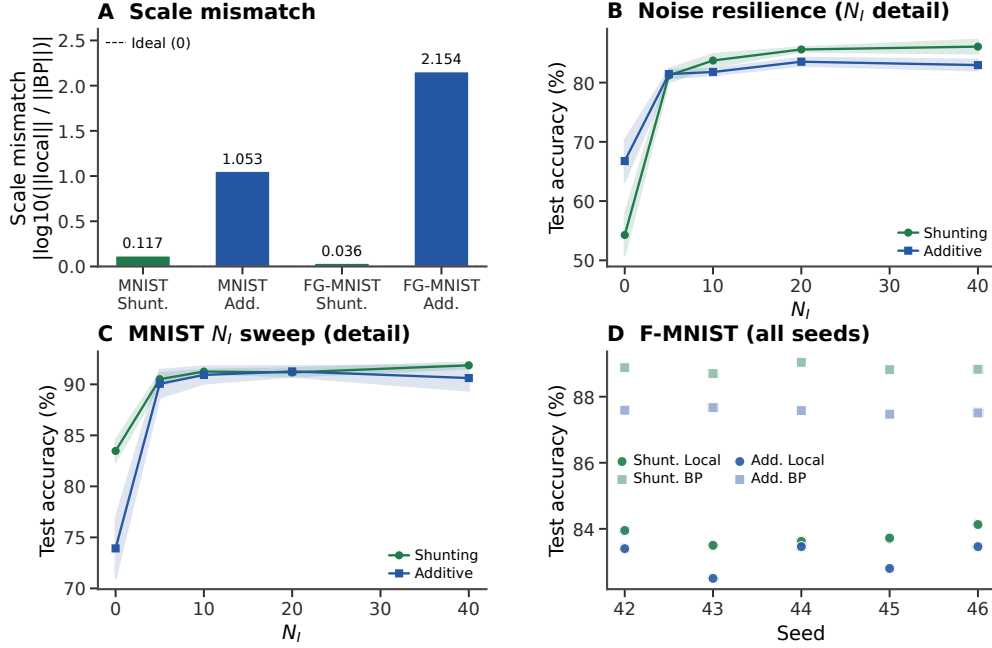
Figure S2: Extended gradient and N_I analysis (supplementary). (A) Log-scale mismatch, |\log_{10}(\|g^{\text{local}}\|/\|g^{\text{bp}}\|)| , from a separate matched-weight static diagnostic; these values should not be compared directly to the checkpointed final-state diagnostic in Fig. 2. The ideal value is 0; shunting is near ideal (0.117), whereas additive shows order-of-magnitude distortion ( > 1.0 ). (B) Noise-resilience N_I dose-response with error bands ( \pm 1 s.d.). (C) MNIST N_I dose-response detail with error bands. (D) Fashion-MNIST individual seeds for all conditions, showing consistency across runs.
