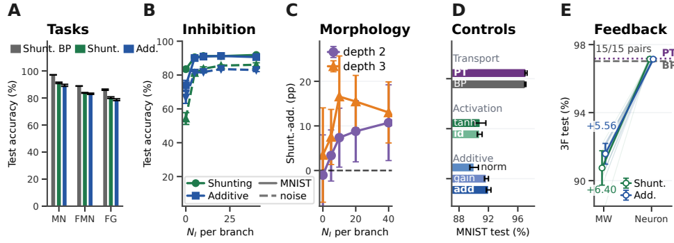
Figure 4: Matched-capacity performance, regime dependence, and feedback correction. (A) Matched shunting backpropagation reference (grey, labelled Shunt. BP) vs. 5F LocalCA with matched-width/scalar-fallback feedback; MN, FMN, and FG denote MNIST, Fashion-MNIST, and figure-ground MNIST. Additive backpropagation references are reported in Table S8 where matched five-seed runs are available. (B) Inhibitory dose-response. (C) Descriptive morphology-by-inhibition performance; the detailed map and its initialization limitation are in Appendix Fig. S10. (D) MNIST controls: BP and exact path transport (PT); learned tanh versus identity transfer (id.); normalized eligibility (+norm); gain-matched additive eligibility (gain); and the additive core (add.). (E) Fifteen-seed 3F intervention: replacing matched-width/scalar-fallback feedback (MW) by one neuron-indexed coordinate shared within each modeled tree raises accuracy by 6.40 points in shunting and 5.56 points in additive networks; all paired seeds improve. Dashed and dotted lines mark the matched shunting BP and exact-transport references. Values/protocols: Table S8; Appendix A. Error bars denote \pm 1 s.d.
