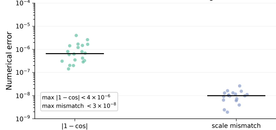
Exact factorization matches autograd
