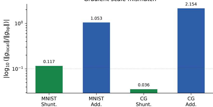
Gradient scale mismatch
