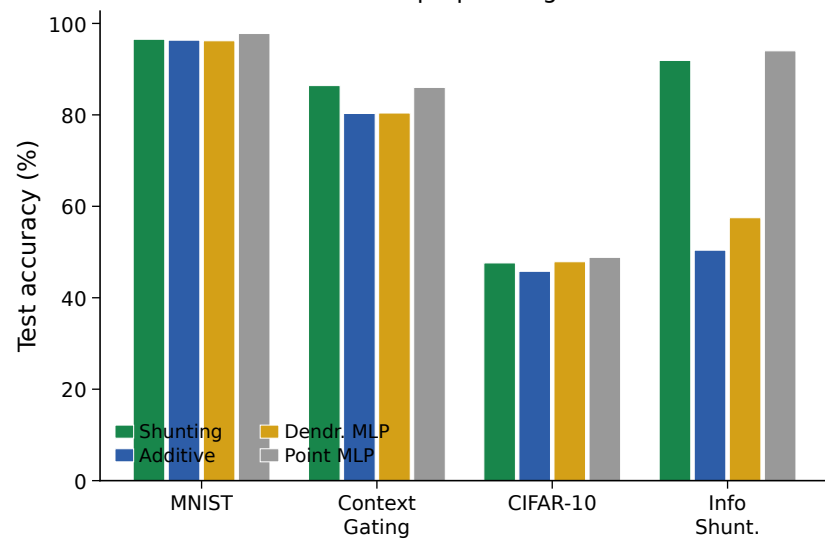
Backprop ceilings
