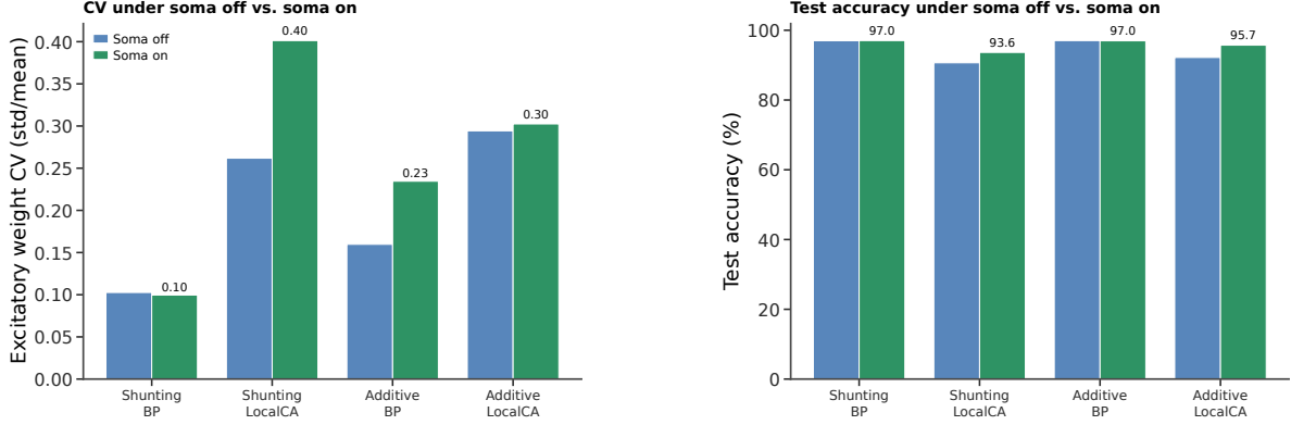
Figure S25: Excitatory-weight CV and MNIST accuracy under soma-off vs. soma-on (depth [3,3], 5 seeds/cell). (A) Coefficient of variation of excitatory weights for the four (core, strategy) cells; paired bars show soma-off (from Fig. S24) and soma-on (this sweep). Shunting + BP tightens slightly; shunting + LocalCA broadens; additive cells change little. (B) Matched MNIST test accuracy (sanity panel). BP accuracy is preserved or marginally improved; LocalCA accuracy is preserved for additive but drops \sim 3 pp for shunting, consistent with the CV widening in panel A.
