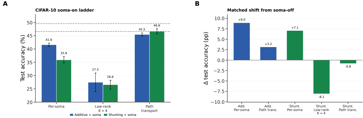
Figure S12: CIFAR-10 compact direct-I-stream depth-4 with somatic_synapses=true . (A) Absolute soma-on ladder on the compact direct-I-stream depth-4 family. Path transport stays strongest in both cores and remains near the matched backprop ceilings (dashed lines), while low-rank K=4 remains weak. (B) Matched shift from soma-off to soma-on for the conditions with a clean paired baseline. Soma helps additive strongly under per-soma and path transport, improves shunting per-soma, leaves shunting transported error close to its soma-off value, and worsens shunting low-rank K=4 . Additive low-rank K=4 is omitted from panel B because the soma-off mechanism package did not include that exact matched condition.
