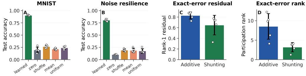
Figure S11: Post-training inhibition intervention and exact-error compressibility . (A,B) Post-training inhibitory-conductance interventions on trained shunting LocalCA checkpoints. Accuracy is measured on a 512-example held-out subset; dots show seeds. Removing, shuffling, or clamping learned inhibition collapses performance, showing that the learned inhibitory field carries sample-specific task structure. (C,D) SVD diagnostics of the exact compartment-error matrix on matched MNIST N_I=5 runs. Shunting has a smaller rank-1 residual and lower participation rank than additive, so the exact error field is more compressible. Error bars are s.d. across 5 seeds.
