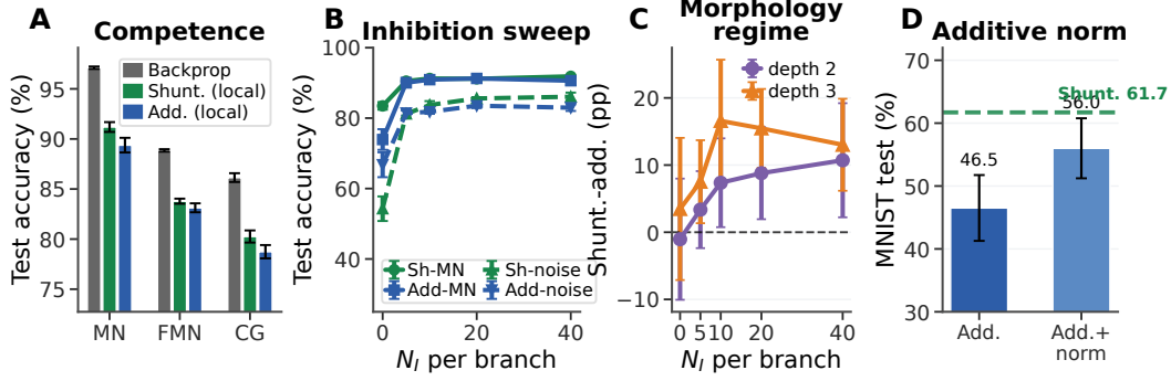
Figure 4: Capacity-calibrated competence and regime dependence. (A) Matched backprop vs. rank-1 5F LocalCA on MNIST, Fashion-MNIST, and context gating. (B) Inhibitory dose-response. (C) Morphology-dependent shunting advantage on noise resilience. (D) Separate stress-regime additive-normalization diagnostic. Error bars denote \pm 1 s.d. where available.
