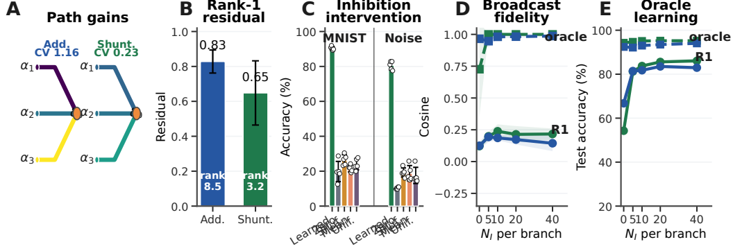
Figure 3: Mechanistic chain from path gains to learning. (A) Path-gain fields at matched inhibition. (B) Exact-error compressibility on MNIST. (C) Post-training inhibitory-conductance interventions (learned, zero, shuffled, mean-clamped, or uniform matched inhibition). (D) Compartment-error fidelity on noise resilience; dashed lines show the [C] transported-error oracle. (E) Transported-error learning where rank-1 broadcast fails. Error bars are \pm 1 s.d.
