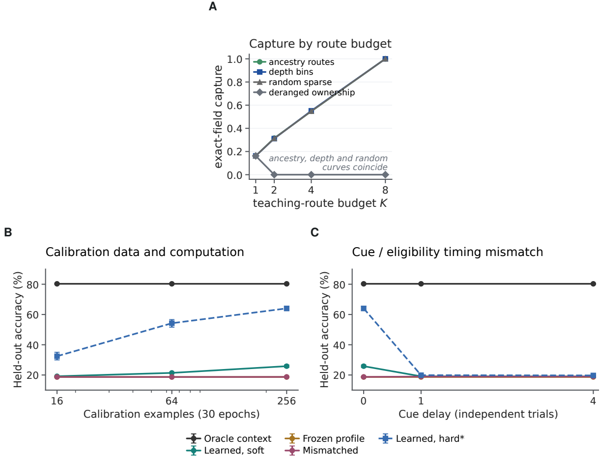
Figure S11: Available route span and learned route coefficients are different constraints. A , Trained field capture by route budget in the eight-context factorial. Ancestry, depth and random partitions have coincident capture at matched bandwidth; derangement removes the target coordinate. Capture therefore does not explain the small ancestry-specific advantage, and capture alone does not predict trained utility: the within-seed Spearman correlation between capture and utility is about 0.82 over all budgets and 0.64 for K < 8 , and is retained numerically in Source Data. B , Held-out accuracy versus calibration set size (16, 64 and 256 examples) at cue-noise standard deviation 0.5 and zero delay; 30 epochs are fixed, so both data and computation increase. C , Cue delay at 256 calibration trials and noise SD 0.5; delays mismatch independent contexts and are measured in trials, not physiological time. In B,C the dashed curves marked with an asterisk use maximum-probability route selection by the same frozen encoder, an exploratory paired sensitivity specified after the soft outcomes with no encoder refit. Curves, diamonds and bars are means and 95% paired-seed bootstrap intervals over twenty fresh analysis seeds. The cue-noise sensitivity of the same encoder is drawn at the main-text type scale in main Fig. 3F. The calibration cue and activation targets are supplied resources. No serial forward dendritic computation is present.
