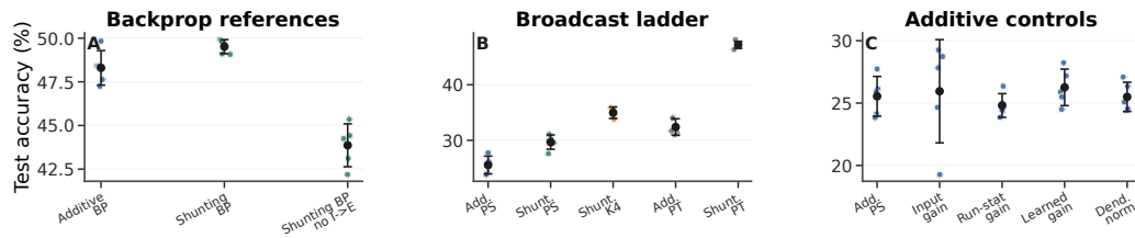
Figure S9: CIFAR-10 control ladder in the compact direct-I-stream family . (A) Matched back-propagation references. With nonnegative inputs and a nonlinear decoder, shunting slightly exceeds additive under standard training, and removing learned I-to-E conductance lowers the shunting reference. (B) Broadcast ladder. The submitted matched-width/scalar-fallback feedback remains weak on this harder dataset, random low-rank K=4 improves partially, and exact effective transported error nearly reaches the matched shunting backpropagation reference. (C) Additive fairness controls. Input-dependent gain, running-stat gain, learned gain, and dendritic normalization do not rescue the additive submitted-feedback baseline. This figure is a harder-dataset stress test, not a claim of competitive CIFAR-10 benchmarking.
