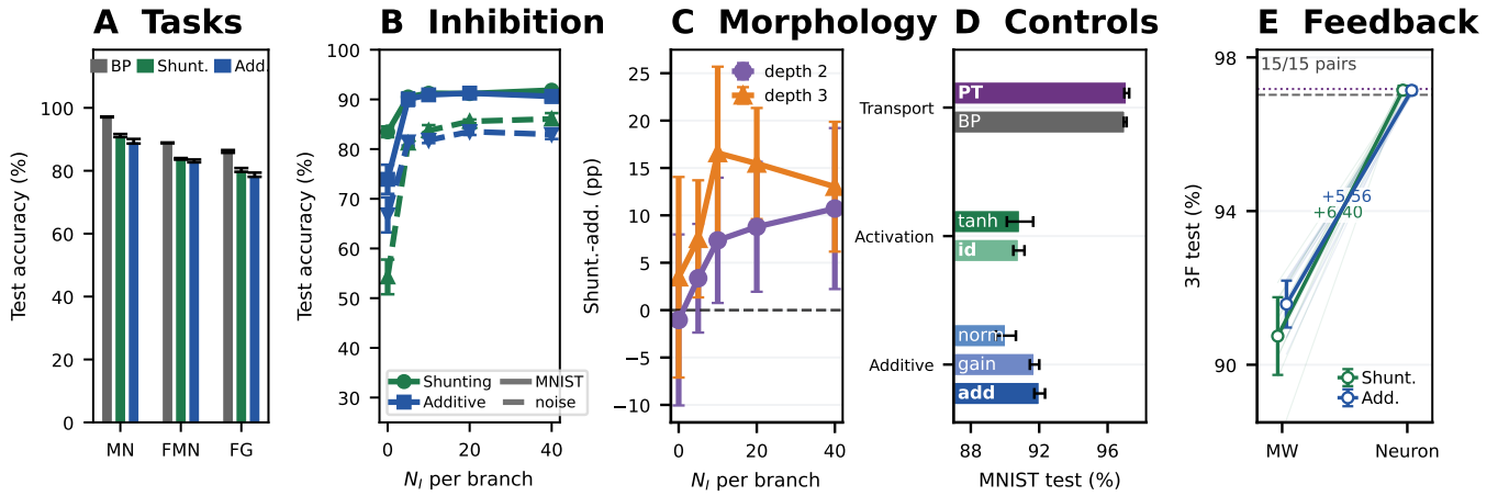
Figure 4: Matched-capacity performance, regime dependence, and feedback correction. (A) Matched shunting backpropagation reference vs. matched-width/scalar-fallback 5F LocalCA; MN, FMN, and FG denote MNIST, Fashion-MNIST, and figure-ground MNIST. Additive backpropagation references are reported in Table S8 where matched five-seed runs are available. (B) Inhibitory dose-response. (C) Descriptive morphology-by-inhibition performance; the detailed map and its initialization limitation are in Appendix Fig. S11. (D) MNIST controls: backpropagation (BP), exact path transport (PT), identity vs. learned tanh activation, and additive gain/normalization variants. (E) Fifteen-seed 3F intervention: replacing matched-width/scalar-fallback feedback (MW) by one neuron-indexed coordinate shared within each modeled tree raises accuracy by 6.40 points in shunting and 5.56 points in additive networks; all paired seeds improve. Dashed and dotted lines mark the matched shunting BP and exact-transport references. Values/protocols: Table S8; Appendix A. Error bars denote \pm 1 s.d.
