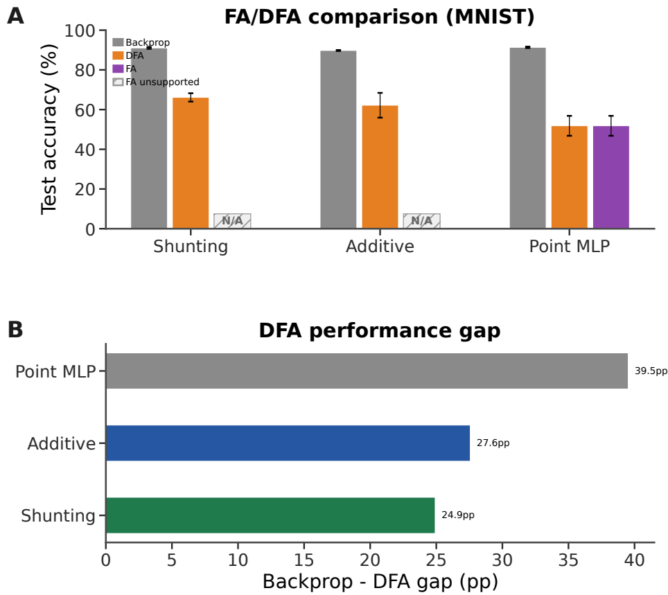
Figure S8: Feedback alignment baselines (MNIST) . (A) Grouped comparison: standard backprop (neutral gray), DFA (orange), and FA (purple). Hatched N/A markers indicate that FA is not implemented for the block-structured dendritic architectures because the random feedback matrices are not dimensionally compatible with the tree-structured branch updates. DFA achieves 66.1% on shunting vs. 62.2% additive vs. 51.8% point MLP. (B) Backprop–DFA gap: dendritic architectures (24.9–27.6 pp) show smaller gaps than point MLPs (39.5 pp), suggesting conductance-based architecture is partially compatible with random feedback.
