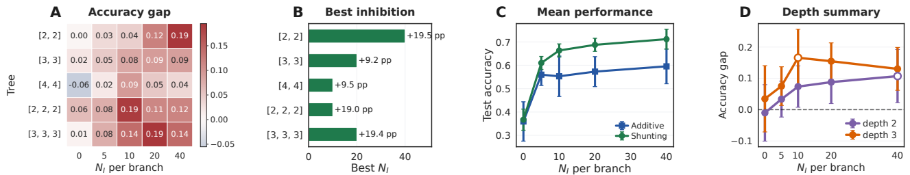
Figure S11: Descriptive morphology \times inhibition performance map . (A) Shunting-minus-additive LocalCA accuracy gap across dendritic morphologies and inhibitory synapse counts. (B) Best inhibitory count for each morphology. (C) Mean performance across tested trees. (D) Average shunting advantage by depth, with markers showing the peak inhibitory count for each depth. The grid uses nonnegative inputs. Because analytical initialization places one shunting population at a near-zero coupling floor, these comparisons are descriptive rather than a causal morphology intervention.
