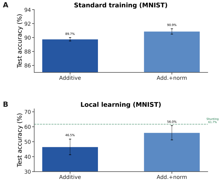
Figure S10: Additive + normalization control (MNIST stress-regime diagnostic) . (A) Standard backprop: normalization provides a small boost (89.7% \rightarrow 90.9%). (B) Local learning: normalization improves additive from 46.5% to 56.0% (+9.5 pp), partially closing the gap to shunting (61.7%, dashed green). These lower local accuracies come from a separate stress-regime diagnostic, not from the matched-capacity performance setting in Table S8.
