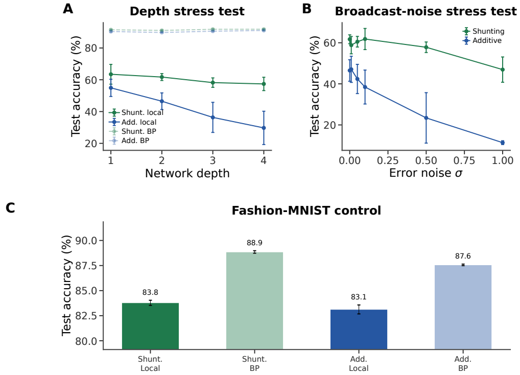
Figure S7: Additional stress tests. (A) Depth scaling: shunting local (green) degrades more gracefully from 63.5% to 57.4%; additive local (blue) drops from 54.9% to 29.7%. Matched backpropagation references (dashed) remain stable. (B) Broadcast-noise robustness: shunting remains stable for \sigma \leq 0.1 ; additive degrades rapidly and reaches chance at \sigma = 1 . (C) Fashion-MNIST: the shunting gain is modest on this cleaner benchmark (83.8% local vs. 88.9% backprop), consistent with the regime-dependent interpretation in the main text.
