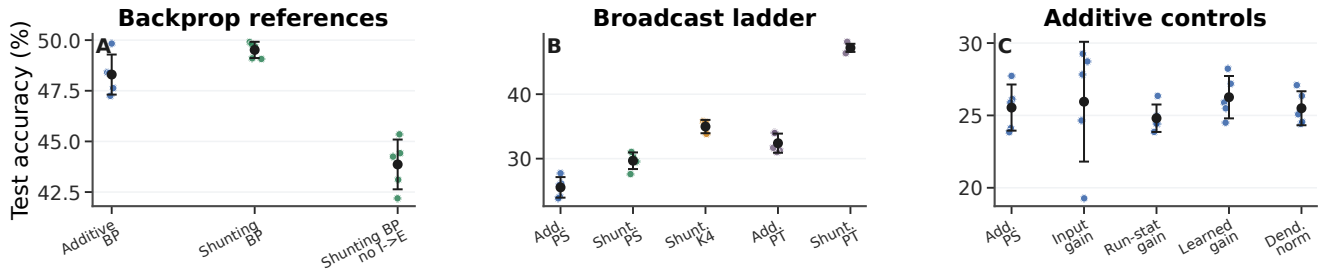
Figure S9: CIFAR-10 control ladder in the compact direct-I-stream family. (A) Matched backpropagation references. With nonnegative inputs and a nonlinear decoder, shunting slightly exceeds additive under standard training, and removing learned I-to-E conductance lowers the shunting reference. (B) Broadcast ladder. The submitted matched-width/scalar-fallback feedback remains weak on this harder dataset, random low-rank K=4 improves partially, and exact effective transported error nearly reaches the matched shunting backpropagation reference. (C) Additive fairness controls. Input-dependent gain, running-stat gain, learned gain, and dendritic normalization do not rescue the additive submitted-feedback baseline. This figure is a harder-dataset stress test, not a claim of competitive CIFAR-10 benchmarking.
