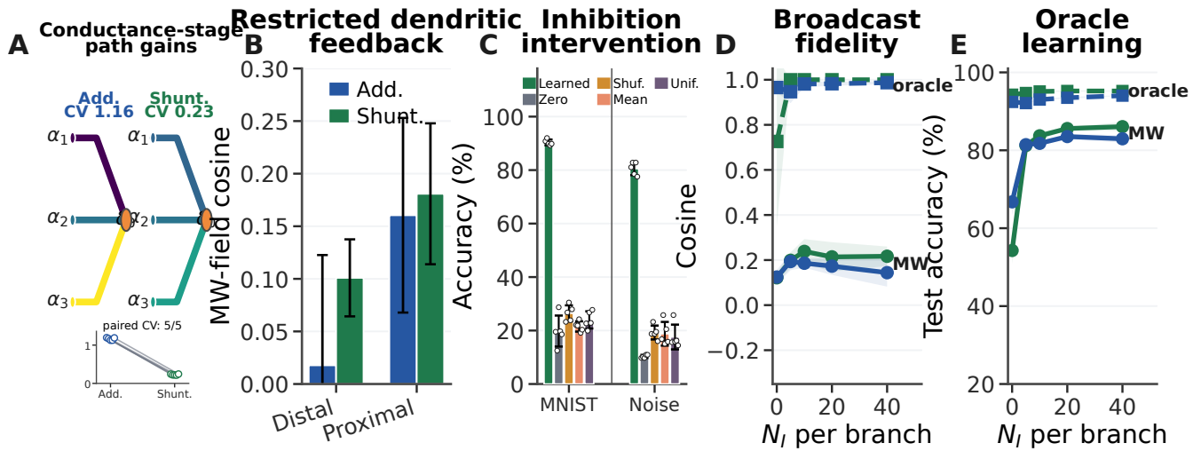
Figure 3: Mechanistic chain from path gains to learning. (A) Conductance-stage path-gain field \alpha^{\text{cond}} at N_l=5 ; the inset shows the five paired-seed CV values, with lower shunting CV in every pair. (B) Stage-resolved cosine between the submitted matched-width/scalar-fallback field and the exact MNIST error on distal and proximal compartments. The width-matched somatic stage is excluded because its cosine is one by construction in both cores. Fidelity is low on both dendritic stages, and the five-checkpoint comparison is descriptive rather than evidence for a cross-core ordering. (C) Post-training inhibitory-conductance interventions. (D,E) Fidelity and learning with matched-width/scalar-fallback feedback (MW) or exact transported error (oracle) on noise resilience. CV denotes the coefficient of variation over the sampled path-gain field and N_l the number of inhibitory synapses per branch. Metrics and interventions: Appendix A. Error bars are \pm 1 s.d.
