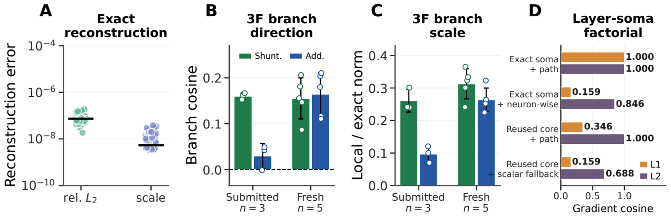
Figure 2: Exact reconstruction and gradient diagnostics. (A) Exact-factorization reconstruction matches autograd. (B,C) Matched 3F parameter-count-weighted branch-gradient cosine and local/exact norm ratio at non-somatic dendritic blocks for the three submitted checkpoint pairs and a fresh five-seed cohort; each dot is one checkpoint averaged over train, validation, and test diagnostic batches. Full values and inference limits are reported in Appendix Tables S9 and S10. (D) Energy-weighted branch-gradient cosine in a layer-soma factorial separating exact vs. reused soma teaching signals, neuron-wise feedback, and exact path transport; L1 and L2 denote dendritic network layers. The two L1 conditions shown as 0.159 differ before rounding. Metrics/protocol: Appendix A. Error bars in (B,C) are \pm 1 s.d. across seeds within each cohort.
