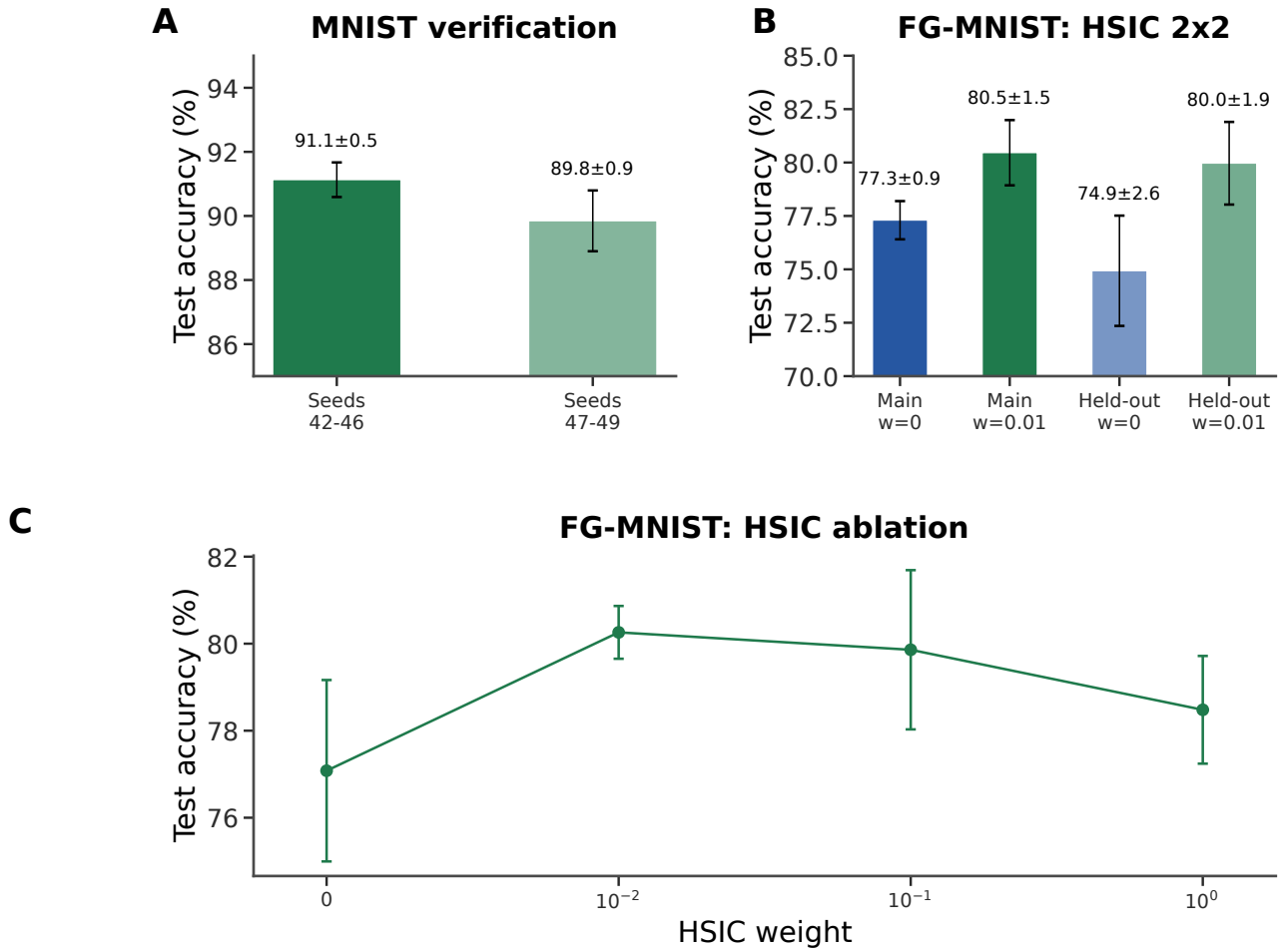
Figure S6: Verification and seed robustness (supplementary). (A) MNIST verification: repeat runs on main seeds (42–46) yield 91.1 \pm 0.5\% ; held-out seeds (47–49) yield 89.8 \pm 0.9\% , showing robustness across random seeds. (B) Matched figure-ground MNIST HSIC control: both main seeds (42–46) and held-out seeds (47–49) compare HSIC weight 0 against 0.01. (C) HSIC weight ablation on figure-ground MNIST: moderate weights (0.01–0.1) perform best.
