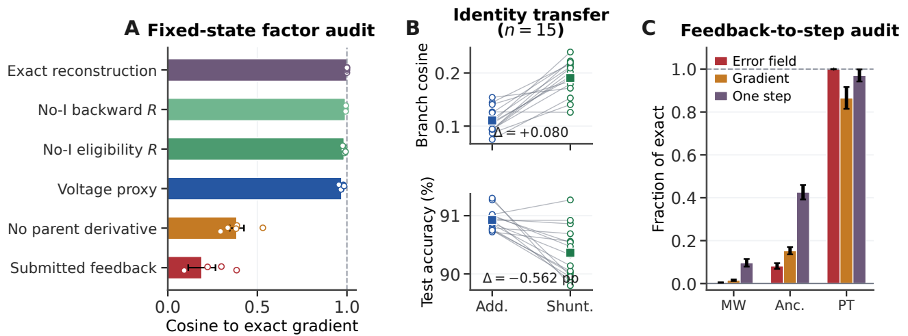
Figure S4: Mechanistic audit separating path effects from learning consequences. (A) Fixed-forward-state factor substitutions in five shunting checkpoints. Removing inhibitory conductance from either resistance factor leaves gradient direction close to exact reconstruction, whereas omitting parent transfer derivatives or using the submitted feedback causes larger directional errors. Bars are mean \pm s.e.m.; points are seeds. (B) Fifteen paired identity-transfer checkpoints. Shunting improves branch-gradient direction, while additive test accuracy remains slightly higher; squares denote means. (C) The same-batch feedback ladder measured as optimally rescaled dendritic error-field capture, eligibility-weighted branch-gradient capture, and norm-matched one-step progress at relative step 10^{-5} . Bars pool five checkpoints per core after averaging three diagnostic splits; error bars are s.e.m. over checkpoints. In this cohort the global scalar equals the submitted field, and the available ancestry field equals exact-soma ancestry. Error geometry alone is therefore not treated as a learning metric. Fixed-state substitutions are diagnostic hybrids, not separately trained forward models.
