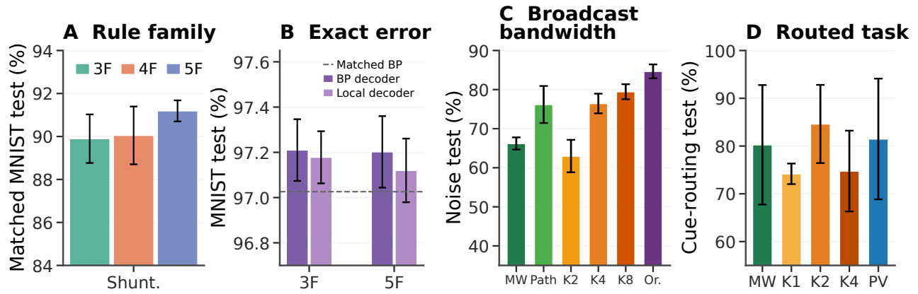
Figure S1: Detailed rule and feedback controls. (A) Within-shunting submitted-code comparison of 3F, 4F, and 5F under matched feedback, decoder, optimizer, and effective parameter-group rates ( n=3 ; descriptive). (B) Five-seed exact-transport factorial: 3F and 5F with a backpropagated or locally updated decoder, with the matched shunting backpropagation reference shown dashed. (C) Feedback-construction ladder on noise resilience: MW submitted feedback, recursive Path, random low-rank K2/K4/K8, and transported Oracle. (D) Cue routing: MW, random low-rank K1/K2/K4, and pathway-vector feedback. The large uncertainty and non-monotonic ordering in (D) make it a boundary result rather than evidence that anatomical routing is optimal.
