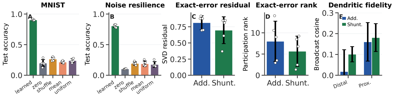
Figure S12: Post-training inhibition intervention and exact-error compressibility. (A,B) Post-training inhibitory-conductance interventions on trained shunting LocalCA checkpoints. Accuracy is measured on a 512-example held-out subset; dots show seeds. Removing, shuffling, or clamping learned inhibition collapses performance, showing that the learned inhibitory field is sample-dependent and functionally important. (C,D) Unrestricted exact-error geometry on matched MNIST N_l=5 runs; these SVD summaries do not test the implemented feedback. (E) Stage-resolved submitted-field cosine on distal and proximal compartments, excluding the exact-by-construction width-matched somatic stage. Error bars are s.d. across 5 seeds.
