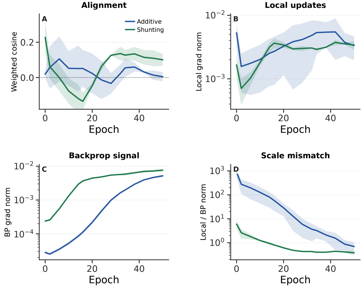
Figure S5: Alignment dynamics with explicit gradient-norm checks. (A) Weighted cosine similarity between LocalCA and backpropagation gradients over training for the 5F rule. (B,C) Weighted local and backprop gradient norms stay nonzero for both additive and shunting models. (D) The additive control begins with a much larger scale mismatch, then approaches the backprop scale without recovering strong directional alignment. Shading is s.d. across 3 seeds.
