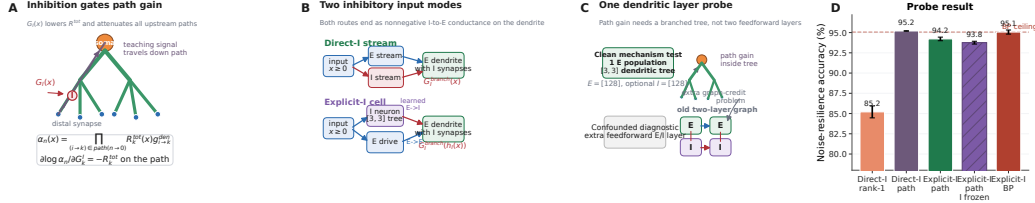
Figure S13: Pathwise inhibition story and one-layer input-mode probe. (A) In a branched conductance tree, the error path gain \alpha_n is the product of local input resistances and dendritic coupling conductances along the path to the soma. Inhibitory conductance on any compartment along that path lowers local input resistance and attenuates all upstream credit paths. (B) The same branch-level inhibitory conductance can be supplied directly from a nonnegative inhibitory input stream ( input_mode=1 ) or through an explicit feedforward inhibitory cell ( input_mode=0 ). (C) The clean mechanism probe keeps the dendritic tree depth ([3, 3]) but uses only one feedforward dendritic population; adding a second feedforward E/I layer tests a deeper graph-credit problem rather than the path-gain mechanism itself. (D) Noise-resilience results for the one-layer probe. Direct-I path transport reaches the explicit-I backprop ceiling, and explicit inhibitory cells with path-transport LocalCA also remain near ceiling. This supports the interpretation that explicit inhibitory cells can generate useful path-gain structure when the architecture isolates the dendritic-path question.
