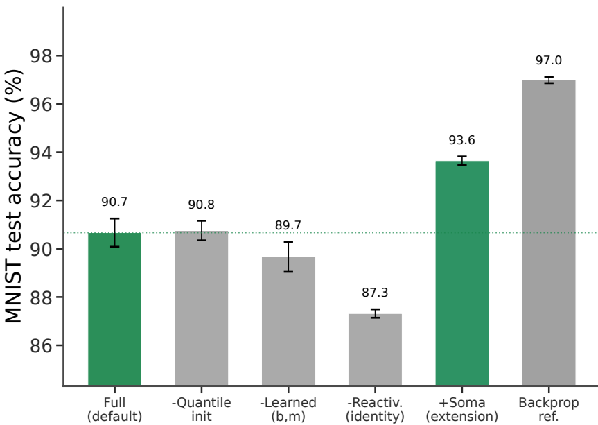
(A) Shunting (MNIST)
