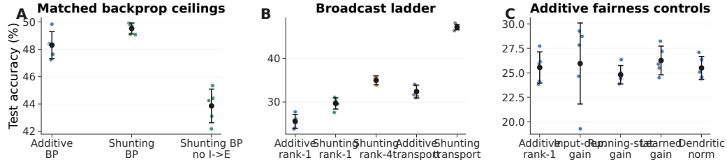
Figure S11: CIFAR-10 control ladder in the compact direct-I-stream family. (A) Matched backprop ceilings. With nonnegative inputs and a nonlinear decoder, shunting slightly exceeds additive under standard training, and removing learned I-to-E conductance lowers the shunting ceiling. (B) Broadcast ladder. Rank-1 broadcast remains weak on this harder dataset, rank-4 improves partially, and exact transported error nearly reaches the shunting backprop ceiling. (C) Additive fairness controls. Input-dependent gain, running-stat gain, learned gain, and dendritic normalization do not rescue additive rank-1 broadcast. This figure is a harder-data diagnostic, not a claim of competitive CIFAR-10 benchmarking.
