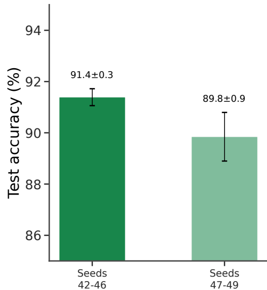
MNIST verification
