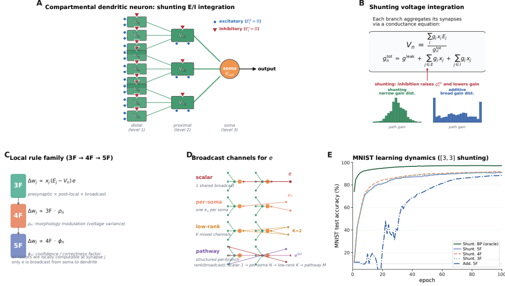
Figure 1: Model and credit assignment. (A) A compartmental dendritic neuron with excitatory (blue circles) and inhibitory (red triangles) synapses arranged on a rooted tree. Voltages propagate to the soma through learned dendritic conductances (green arrows), which is the operating regime studied in the main feedforward experiments. (B) Shunting voltage integration. The branch voltage is set by a conductance equation in which inhibition enters the denominator; the paired histograms illustrate the visual intuition behind the paper, namely that shunting narrows the conductance-stage path-gain distribution while additive integration leaves it broad. (C) LocalCA rule hierarchy. 3F is the theorem-facing rule, 4F adds the heuristic morphology-aware factor \rho , and 5F adds the heuristic confidence-like factor \phi . (D) Broadcast modes. Scalar sends one shared field, per-soma sends an output-space vector when dimensions match and otherwise falls back to scalar, random low-rank adds a few unstructured channels, and structured pathway feedback preserves pathway identity when branches should receive different teaching signals. (E) Representative MNIST learning dynamics from the fixed-epoch Figure 1 sweep. Shunting with the stronger local wrappers tracks backprop much more closely than the additive control, giving a concrete preview before the paper turns to the sharper gradient-fidelity diagnostics in Fig. 2.
