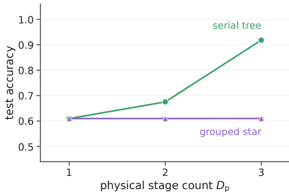
Serial composition
