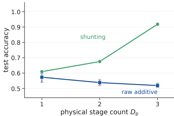
Divisive control
