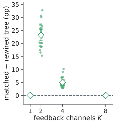
Task-topology alignment
