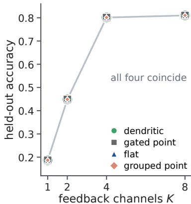
Representation match
