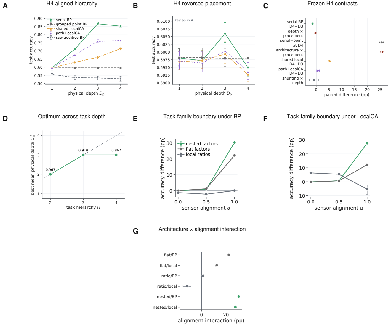
Figure 6: Depth saturation and task-family crossovers bound when serial dendritic composition helps. A,B, Accuracy across D1–D4 under aligned and reversed sensor placement for serial BP, literal grouped-point BP, shared-soma LocalCA, exact-path LocalCA and the aligned raw-additive control. C, Seed-paired frozen primary contrasts; positive values favor the first named condition. D, Best mean trained physical depth across the clean-source H2/H3 cohorts and the frozen H4 cohort. The diagonal is one-to-one tracking; D3, not D4, maximizes H4 exact-BP accuracy. All H4 conditions use paired seeds 10400–10409; lines and intervals are means and 95% seed-bootstrap intervals, and primary-family P values are BH corrected. E,F, Serial-minus-literal-grouped-point accuracy across task–sensor alignment for nested factors, flat factors and local ratios under BP and path-transport LocalCA. G, The paired \alpha = 1 minus 0 architecture interaction. Panels E–G use ten paired seeds 10500–10509; points and bars are means and 95% paired-seed bootstrap intervals.
