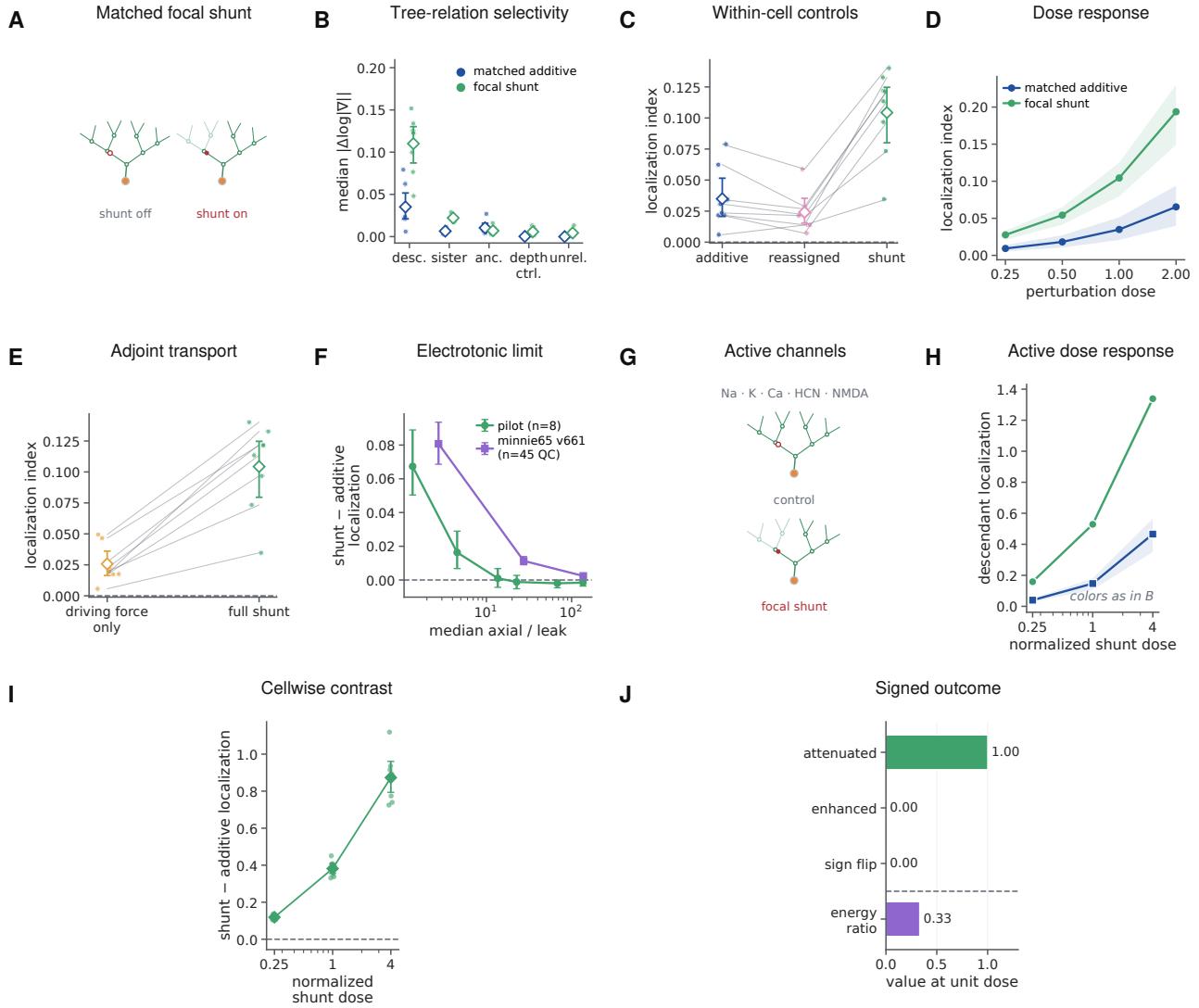
Figure 8: Focal shunting produces a descendant-enriched modeled-credit signature in defined electrotonic regimes. A , Focal intervention with state-matching somatic current, shown as a shunt-off/shunt-on tree pair; the faded descendant subtree marks where the shunt attenuates transported credit. B , Absolute gradient change across tree relations. C , Within-cell localization for the matched additive perturbation, route reassignment and focal shunting. D , Dose response. E , Exact factor-freeze comparison isolating changed adjoint transport. F , Shunt-minus-additive localization across the cable-calibrated axial-to-leak ratio; the standard high-resistance calibration is effectively null. G , Active-channel steady-state design. H,I , Active- model dose response and paired shunt-minus-additive localization. J , Descendant outcomes at unit dose: attenuation, enhancement, sign reversal and residual gradient energy. Points are reconstructed-cell means after averaging sites and channel draws; lines, bands and intervals are 95% cell-bootstrap summaries. The reconstructed cell is the inferential unit. Active validation uses the permissive electrotonic regime and does not restore the effect at the standard passive calibration.
