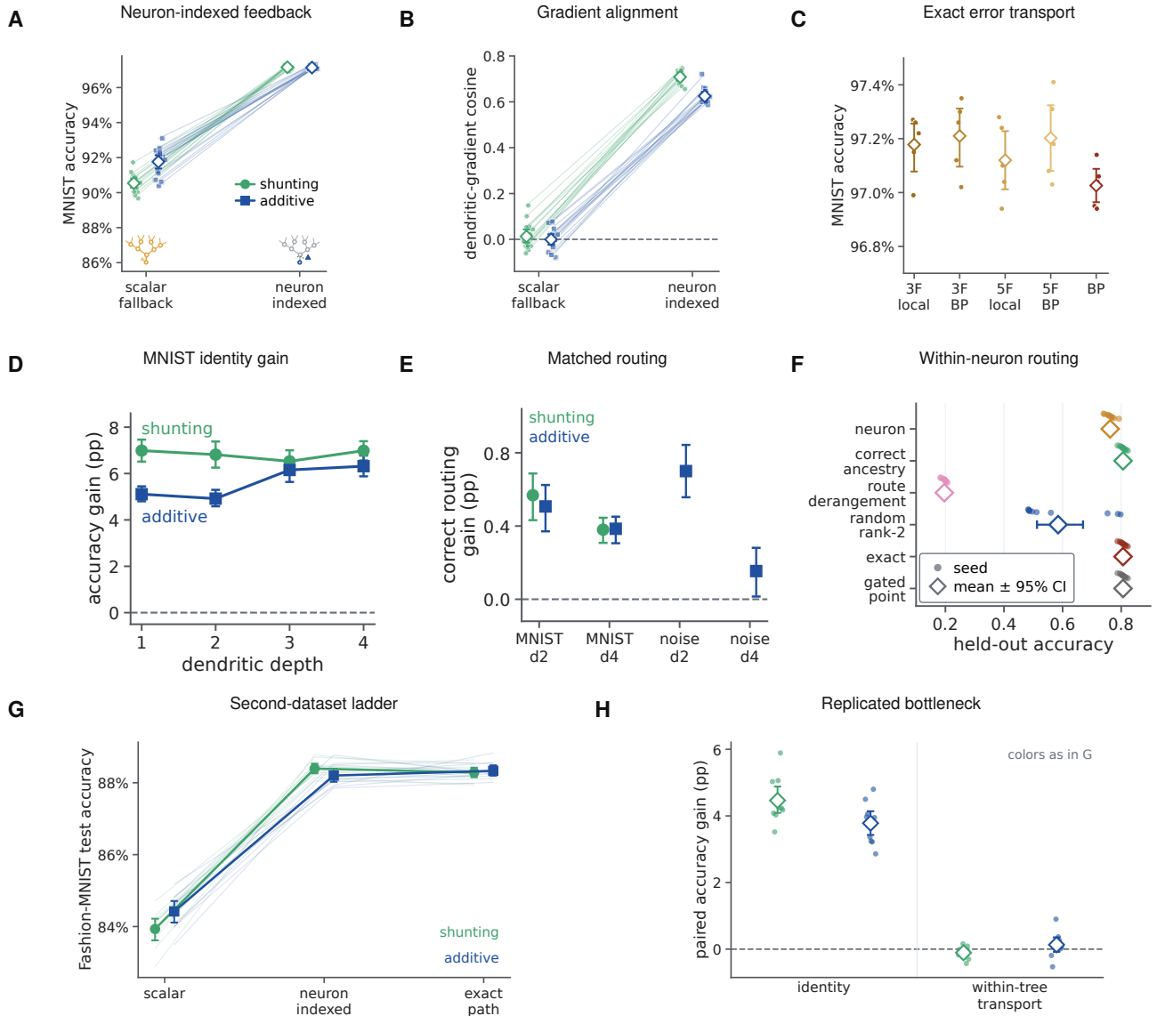
Figure 2: Neuron identity is the dominant feedback bottleneck, with a smaller cost for incorrect route ownership. A , MNIST accuracy under the matched-width/scalar-fallback rule or a neuron-indexed coordinate. B , Exact-gradient cosine at matched checkpoints. C , Accuracy under exact path transport, local rules and backpropagation (BP); exact transport is an information oracle. D , Neuron-indexed-minus-scalar accuracy across dendritic depth in the prospective MNIST cohort. E , Gain from correct rather than deranged neuron-to-tree ownership at matched bandwidth. F , Held-out accuracy in the two-stream credit-reversal task, where the same neuronal error requires different updates in sibling subtrees. G,H , Fashion-MNIST replication of the scalar, neuron-indexed and exact-path ladder and their paired contrasts. Faint lines or small points are paired seeds; large symbols and bars are means and 95% seed-bootstrap intervals. Exact transport, gated-point and correct-subtree-routing values coincide in the shallow representation-matched condition in F .
