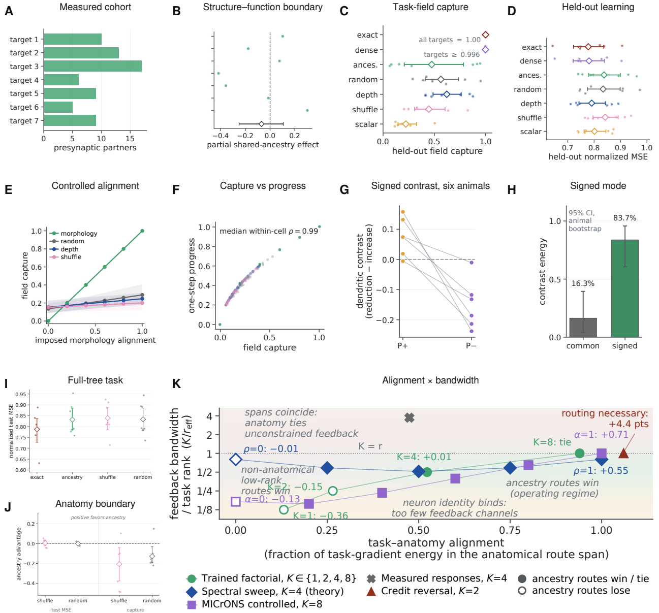
Figure 9: Measured responses define the biological boundary, while imposed alignment validates the conditional prediction. A,B , Seven-cell measured-response cohort and the geometry-controlled structure–function effect. C,D , Held-out task-field capture and learning for exact, dense, ancestry and matched control dictionaries; projection coefficients are oracle ceilings. E,F , Rotating task credit into the fixed ancestry span increases its capture, and capture predicts one-step progress. G , Signed neuron-coordinate contrast in six animals: P+ and P- are defined by the causal experimental mapping. H , Most contrast energy lies in the signed P+/P- mode rather than a common scalar mode. I,J , Complete-tree learning and ancestry-minus-control contrasts across all eligible scans; neither shows a morphology-specific benefit. K , Alignment-by-bandwidth synthesis across trained and controlled experiments; both axes and every plotted coordinate are defined in Methods. Filled markers denote an ancestry win or tie; open markers denote a loss. Coincident markers at full alignment are horizontally offset. Shaded regions summarize the credit-operator regimes and are not fitted to the displayed outcomes. Target cells or animals are the inferential units; nested splits and simulations are averaged within them.
