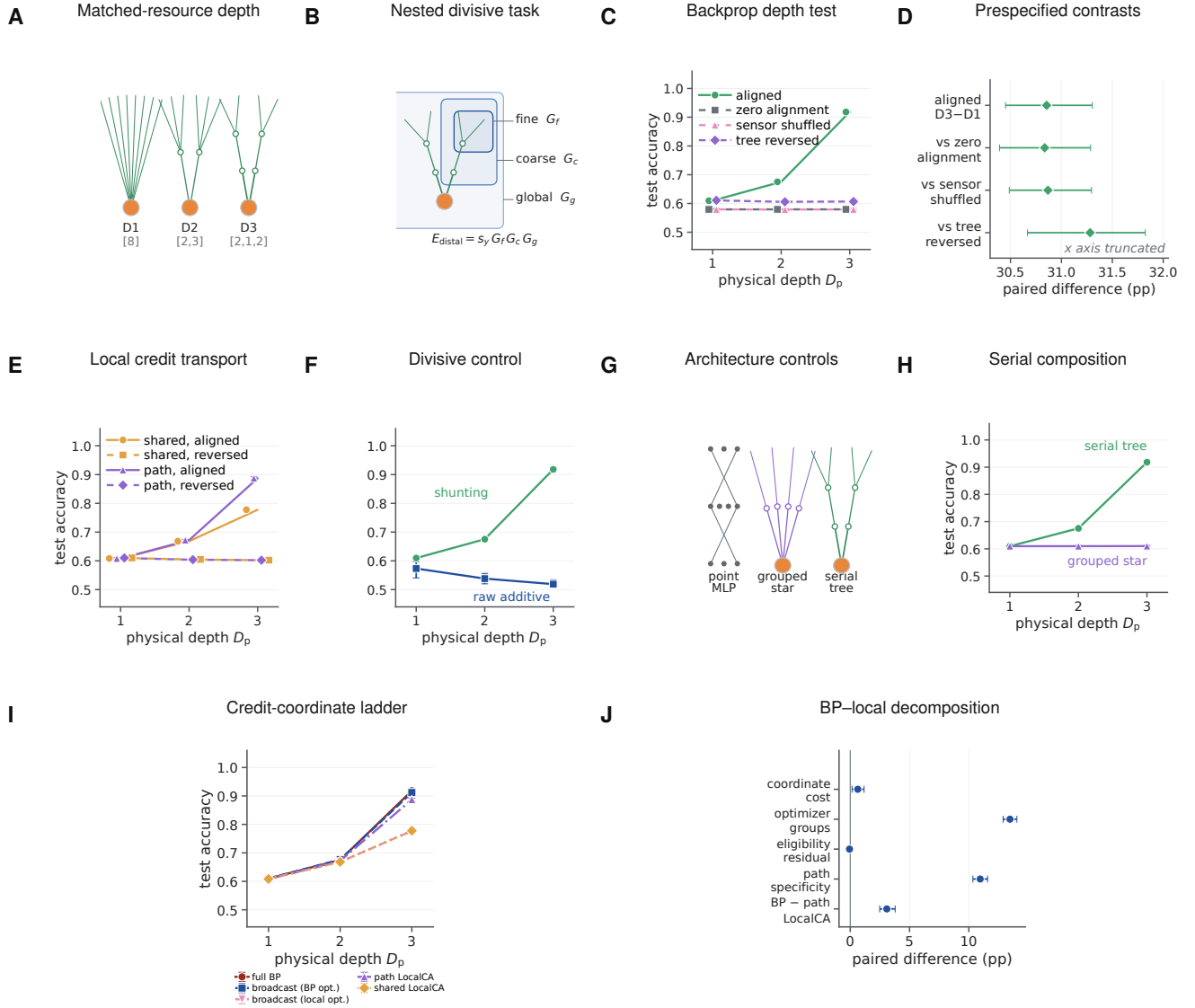
Figure 5: Matched nonlinear hierarchy makes exact-resource physical dendritic depth useful. A , D1–D3 have D_p = 1, 2, 3 stages. Bracket entries are soma-to-distal branching factors: [8], [2, 3] and [2, 1, 2] give 8, 2 + 6 and 2 + 2 + 4 nonsomatic branch units, with identical contact, candidate-slot, parameter and state budgets. B , A distal positive-rate signal is multiplied by fine, coarse and global gains; independent sensors, trial-shuffled sensors and reversed physical placement are matched controls. C , Test accuracy under shunting backpropagation; coincident flat-control markers in C , E , F are offset. D , Prespecified paired D3-minus-D1 effect and aligned-minus-control interactions; bars are 95% paired-seed bootstrap intervals, all excluding zero. E , Aligned and reversed-placement LocalCA with one shared-soma coordinate or exact path transport; the coincident reversed curves are drawn with offset markers. F , Aligned shunting and raw-additive BP. G , Architecture controls that separate a flexible point multilayer perceptron, a nonserial grouped star and the serial tree. H , Serial-tree and grouped-star accuracy across physical depth. I , Credit-coordinate ladder from full BP through soma-broadcast autograd to shared- and path-transport LocalCA. J , Paired D3 decomposition of the BP-local gap into coordinate, optimizer, eligibility and path-specificity contrasts. All inferential runs use paired seeds 10200–10209; lines are seed means and error bars are 95% seed-bootstrap intervals.
