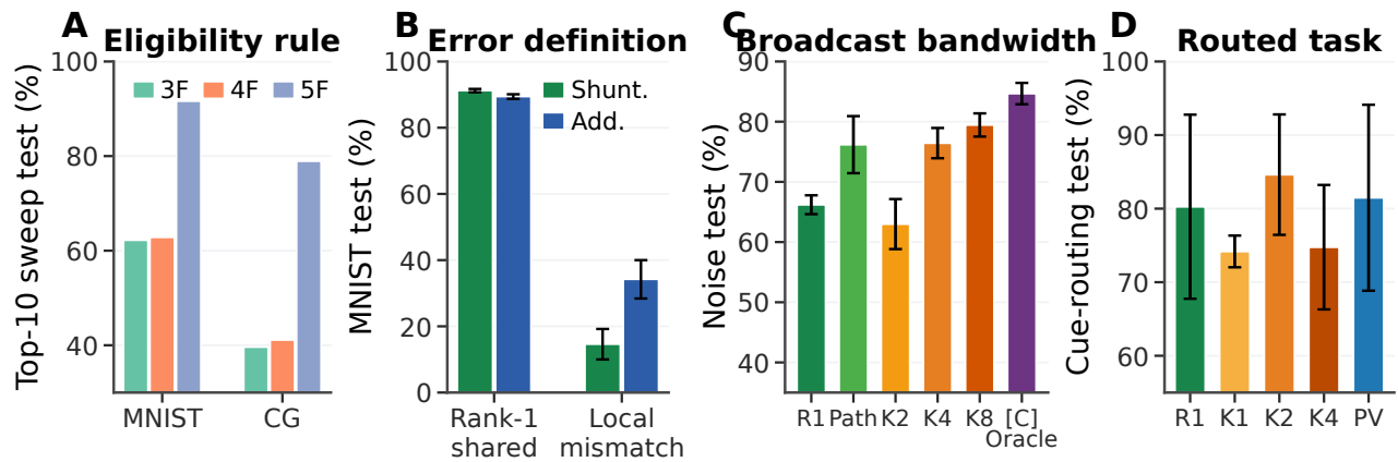
Figure S1: Rule and feedback controls. (A) Eligibility-rule ablation: 3F, 4F, and 5F. (B) Error-source ablation: rank-1 somatic error vs. local mismatch. (C) Feedback-bandwidth ladder on noise resilience: R1, recursive Path, K2/K4/K8, and [C] transported Oracle. (D) Cue routing: rank-1, random low-rank K1/K2/K4, and pathway-vector feedback.
