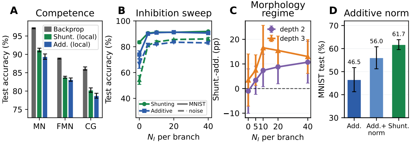
Figure 4: Capacity-calibrated competence and regime dependence. (A) Matched backprop vs. rank-1 5F LocalCA on MNIST, Fashion-MNIST, and context gating. (B) Inhibitory dose-response. (C) Morphology-dependent shunting advantage on noise resilience. (D) Separate stress-regime additive-normalization diagnostic. Error bars denote \pm 1 s.d. where available.
