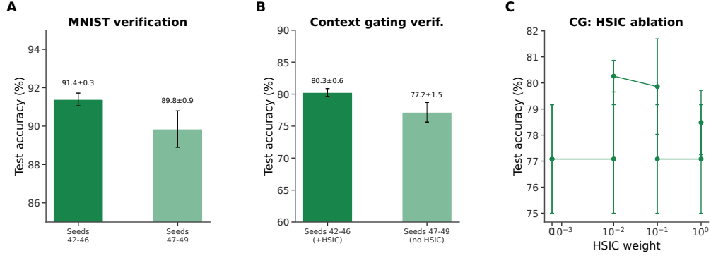
Figure S7: Verification and reproducibility (supplementary). (A) MNIST verification: main seeds (42–46) yield 91.4 \pm 0.3\% ; held-out seeds (47–49) yield 89.8 \pm 0.9\% , confirming generalization. (B) Context gating verification: main seeds (+HSIC) 80.3 \pm 0.6\% ; held-out seeds (no HSIC) 77.2 \pm 1.5\% . The roughly 3 pp gap reflects HSIC removal, not seed sensitivity. (C) HSIC weight ablation on context gating: moderate weights (0.01–0.1) perform best.
