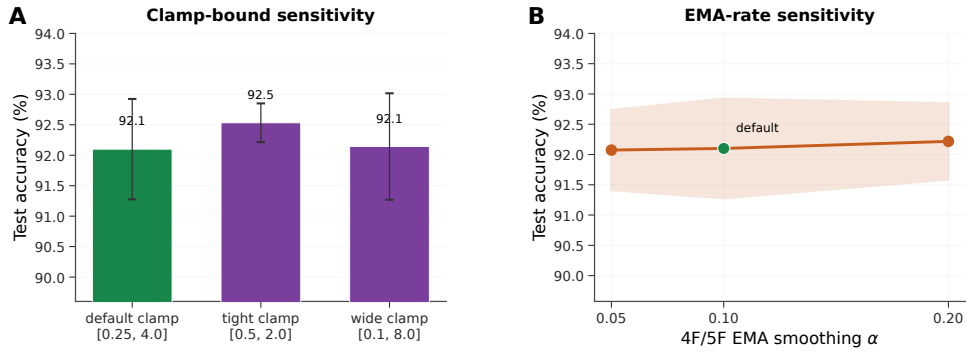
Figure S6: 5F sensitivity analysis (MNIST, shunting, per-soma broadcast). (A) Sensitivity to the \phi_n clamp interval. The default clamp [0.25, 4.0] is already strong ( 92.1 \pm 0.8\% ); tightening it to [0.5, 2.0] slightly improves performance ( 92.5 \pm 0.3\% ), while widening it to [0.1, 8.0] is effectively neutral ( 92.1 \pm 0.9\% ). (B) Sensitivity to the 4F/5F EMA rate used for online statistics. Varying \eta_{\text{ema}} from 0.05 to 0.20 changes mean test accuracy by less than 0.2 pp. Together these results suggest that the 5F gain is not driven by a brittle single hyperparameter choice, even though the factor itself remains heuristic. Errors: \pm 1 s.d. across 3 seeds.
