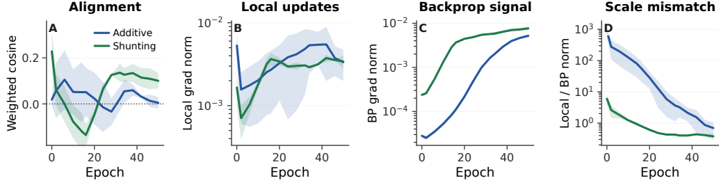
Figure S5: Alignment dynamics with explicit gradient-norm checks. (A) Weighted LocalCA-vs.-backprop cosine over training for the 5F rule. (B,C) Weighted local and backprop gradient norms stay nonzero for both additive and shunting models. (D) The additive control begins with a much larger scale mismatch, then approaches the backprop scale without recovering strong directional alignment. Shading is s.d. across 3 seeds.
