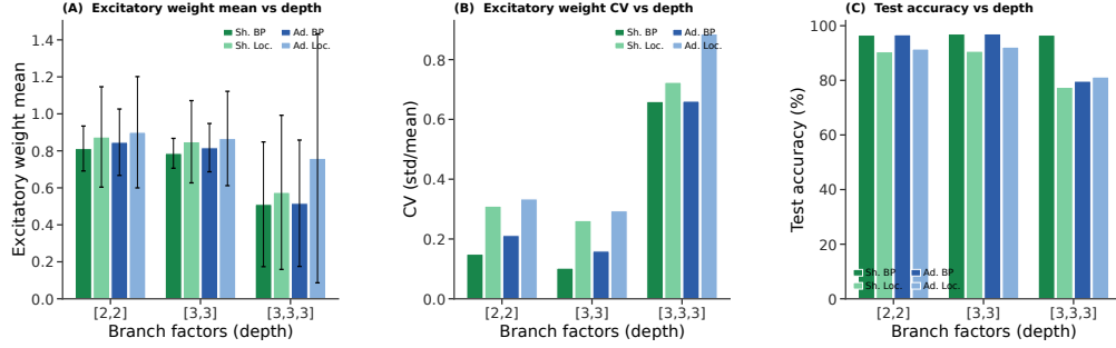
Figure S24: Synaptic weight statistics vs. dendritic depth (MNIST, 5 seeds/cell). (A) Excitatory weight mean (error bars = std). At [2, 2] and [3, 3], all four conditions cluster around 0.8–0.9; at [3, 3, 3] the means drop to \approx 0.5 –0.75 and the cross-seed spread grows, especially for additive LocalCA. (B) Coefficient of variation (CV = std/mean). At shallow/medium depth, LocalCA produces \sim 2\times higher CV than matched BP, but both remain well-behaved ( \leq 0.33 ). At the deepest network all four conditions jump to CV \approx 0.66 –0.88, with additive LocalCA the broadest. (C) MNIST test accuracy. BP tracks \sim 96 –97% at [2, 2]/[3, 3] and \sim 92 –95% at [3, 3, 3]. LocalCA stays within \sim 5 –6 pp of BP at shallow/medium depth but trails by \sim 15 –20 pp at [3, 3, 3], identifying depth as the remaining open challenge for this local rule. The qualitative ordering (shunting LocalCA tracks shunting BP more closely than additive LocalCA tracks additive BP) reinforces the manuscript claim that the conductance denominator is the key mechanistic ingredient.
