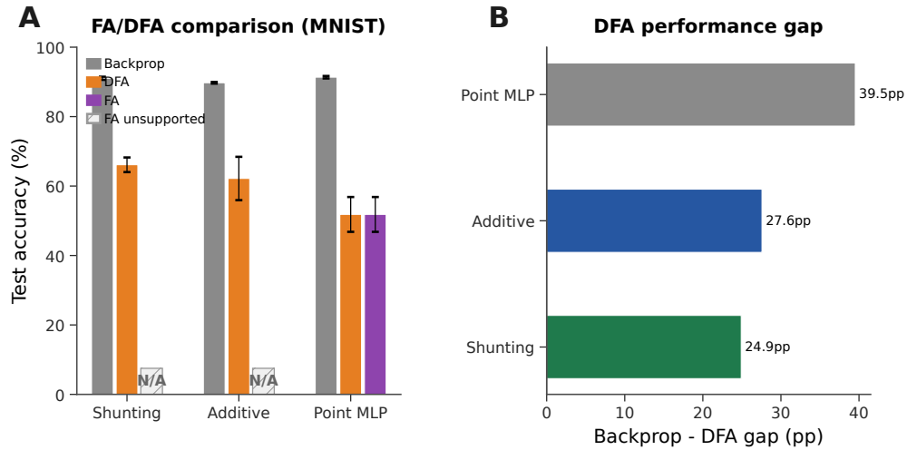
Figure S10: Feedback alignment baselines (MNIST). (A) Grouped comparison: standard backprop (neutral gray), DFA (orange), and FA (purple). Hatched N/A markers indicate that FA is not implemented for the block-structured dendritic architectures because the random feedback matrices are not dimensionally compatible with the tree-structured branch updates. DFA achieves 66.1% on shunting vs. 62.2% additive vs. 51.8% point MLP. (B) Backprop–DFA gap: dendritic architectures (24.9–27.6 pp) show smaller gaps than point MLPs (39.5 pp), suggesting conductance-based architecture is partially compatible with random feedback.
