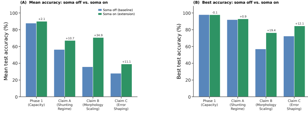
Figure S19: Soma-on extension for LocalCA. Enabling direct somatic input ( somatic_synapses=true ) improves aggregate mean test accuracy across all four manuscript LocalCA families. Each family is summarized over the completed configurations in matched soma-off and soma-on sweeps. The largest gain appears in morphology scaling, where the family mean rises from 35.8% to 70.7% and the best run rises from 57.0% to 76.4%. Gains in the shunting-regime and error-shaping families are smaller but still substantial. Delta labels show soma-on minus soma-off. Because the main mechanistic analysis was developed in the dendrite-only feedforward regime, we report soma-on as a supportive extension rather than replacing the main operating regime.
