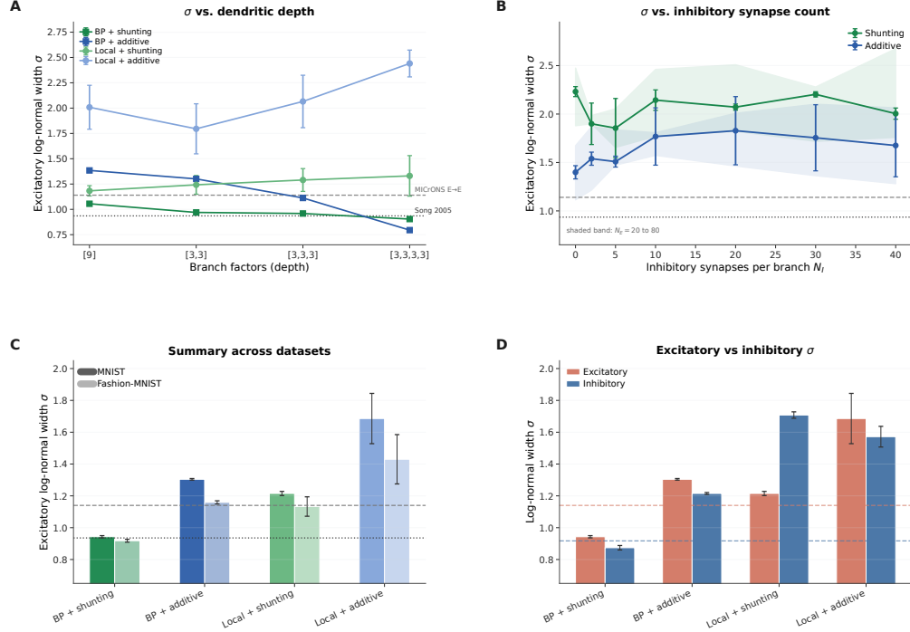
Figure S23: Synaptic weight distribution sensitivity to architecture. (A) Log-normal \sigma vs. dendritic depth (branch factors [9] to [3,3,3,3]). Both backprop and local shunting remain closer to the biological-width references than their additive counterparts across depth. (B) \sigma vs. inhibitory synapses per branch ( N_I ). Without inhibition ( N_I=0 ), all conditions are overly broad; with biologically constrained N_I=10 –20, shunting enters the biological range. Shaded bands show the sweep over N_E=20 to 80. (C) Summary of MNIST and Fashion-MNIST results with biological references. The shunting ordering is consistent across datasets. (D) Excitatory vs. inhibitory weight \sigma on MNIST with MICrONS E→E and I→E reference bands.
