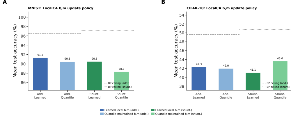
Figure S21: (b, m) update policy under quantile initialization. Each cluster of bars compares the mean test accuracy of learned local (b, m) and quantile-maintained (b, m) under LocalCA for additive and shunting cores, averaged across a matched morphology/init grid ([2, 2] and [3, 3, 3] ; analytical and quantile init variants). Dashed and dotted horizontal lines mark the matched standard backpropagation ceiling for additive and shunting respectively. Left (MNIST): Learned local (b, m) is consistently better; quantile-maintained lags by 1.9 pp (additive) and 3.4 pp (shunting) on mean accuracy. Right (CIFAR-10): The gap reverses for shunting: quantile-maintained reaches 43.6% mean vs. 40.3% for learned local, while additive is essentially tied. The pattern suggests that quantile-maintained (b, m) prevents over-fitting the reactivation gate on harder inputs, making it a useful alternative in harder visual regimes.
