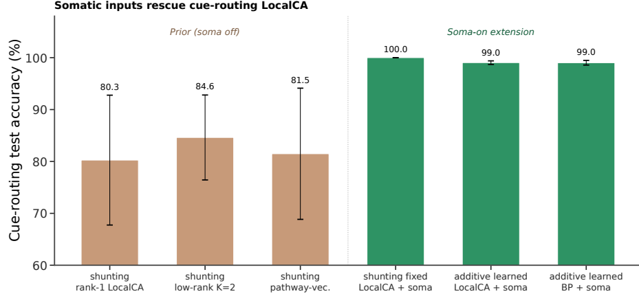
Figure S20: Soma-on rescues cue-routing LocalCA. The left bars show the previously reported soma-off LocalCA results on the cue-integration benchmark. The right bars show the soma-on extension: fixed-router shunting LocalCA reaches 1.00 test accuracy, and learned-router additive LocalCA with soma reaches 0.99, matching the additive backprop ceiling with soma. The soma channel supplies a direct high-bandwidth input that bypasses the rank-1 bottleneck identified in the main text. Learned-router shunting with soma is omitted because this benchmark uses signed cues, which conflict with the shunting positive-input check in the learned-router pipeline; fixed-router shunting is therefore the clean shunting data point.
