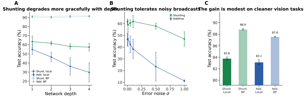
Figure S8: Additional stress tests. (A) Depth scaling: shunting local (green) degrades more gracefully from 63.5% to 57.4%; additive local (blue) drops from 54.9% to 29.7%. Backprop ceilings (dashed) remain stable. (B) Broadcast-noise robustness: shunting remains stable for \sigma \leq 0.1 ; additive degrades rapidly and reaches chance at \sigma = 1 . (C) Fashion-MNIST: the shunting gain is modest on this cleaner benchmark (83.8% local vs. 88.9% backprop), consistent with the regime-dependent story in the main text.
