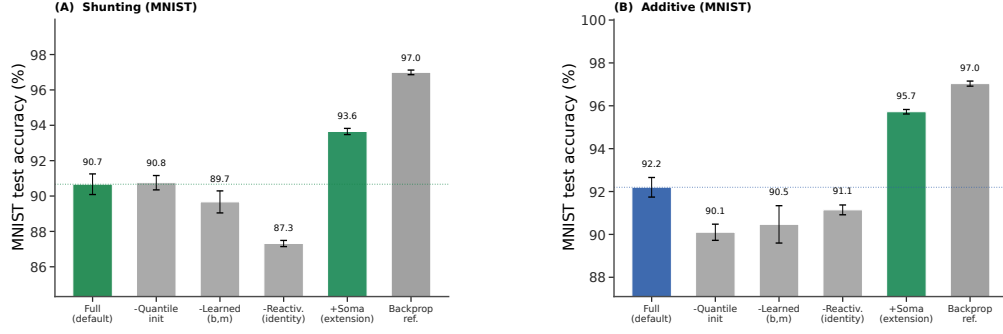
Figure S22: Per-component ablation for LocalCA on MNIST. Bars show mean test accuracy ( \pm s.d. across 5 seeds); coloured bars highlight the manuscript default (blue/green) and the soma-on extension (green). (A) Shunting: The full default reaches 90.7%; removing quantile init leaves accuracy unchanged at 90.8% (quantile init is a mild calibration nudge on this clean task), removing learned ( b, m ) drops by about 1 pp, and removing reactivation entirely drops accuracy to 87.3%; the reactivation transform is the largest single LocalCA ingredient. (B) Additive: Quantile init contributes +2.1 pp (90.1 \rightarrow 92.2%), learned ( b, m ) contributes +1.7 pp, and reactivation contributes +1.1 pp; each ingredient helps on the additive core. Soma-on is the largest positive change in both cores (+3 to +3.5 pp over full config), while matched standard backpropagation reaches 97.0% in both cores and sets the upper reference. The fixed-relu reactivation condition did not satisfy the same initialization checks and is omitted.
