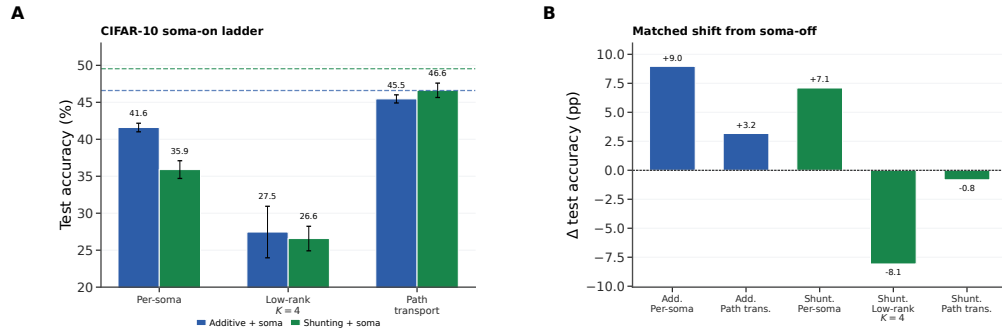
Figure S12: CIFAR-10 compact direct-I-stream depth-4 with somatic_synapses=true. (A) Absolute soma-on ladder on the compact direct-I-stream depth-4 family. Path transport stays strongest in both cores and remains near the matched backprop ceilings (dashed lines), while low-rank K=4 remains weak. (B) Matched shift from soma-off to soma-on for the conditions with a clean paired baseline. Soma helps additive strongly under per-soma and path transport, improves shunting per-soma, leaves shunting transported error close to its soma-off value, and worsens shunting low-rank K=4 . Additive low-rank K=4 is omitted from panel B because the soma-off mechanism package did not include that exact matched condition.
