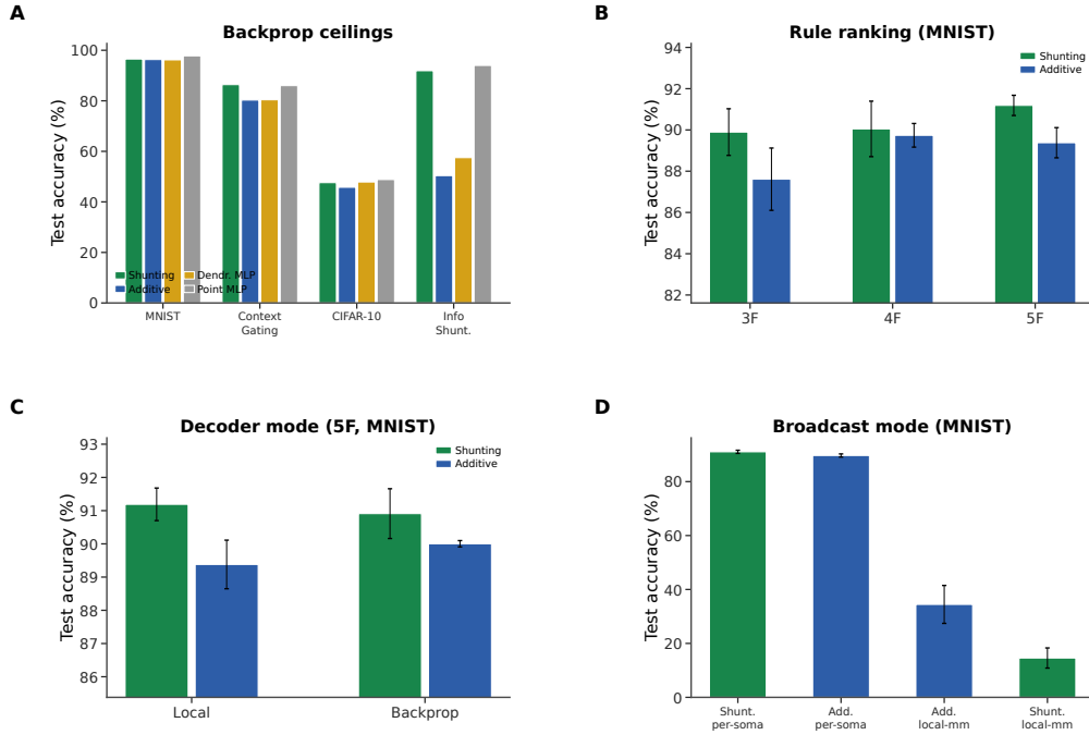
Figure S3: Capacity calibration (supplementary) . (A) Phase 1 backprop ceilings across all architectures and datasets. (B) Rule-family ranking: 5F consistently outperforms 4F and 3F. (C) Decoder mode comparison (local vs. backprop decoder, 5F MNIST). (D) Broadcast mode comparison: the historical per_soma mode/rank-1 fallback is required for strong performance; local-mismatch fails.
