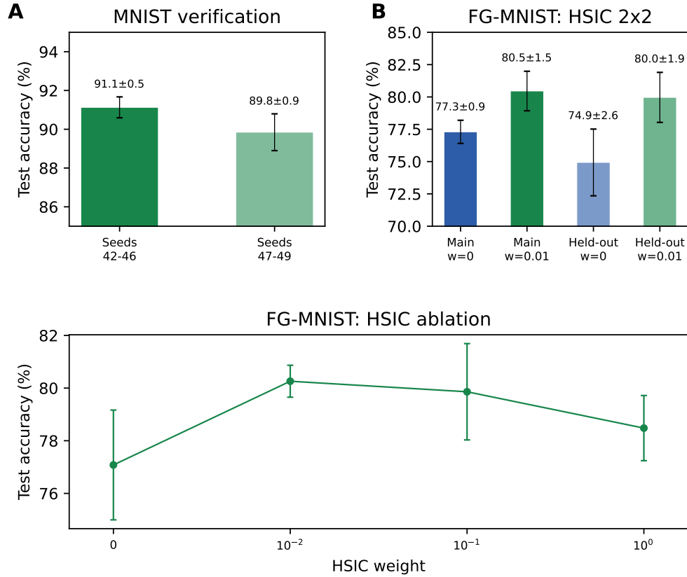
Figure S5: Verification and reproducibility (supplementary). (A) MNIST verification: the current-code rerun of main seeds (42–46) yields 91.1 \pm 0.5\% ; held-out seeds (47–49) yield 89.8 \pm 0.9\% , showing robustness across random seeds. (B) Matched figure-ground MNIST HSIC control: both main seeds (42–46) and held-out seeds (47–49) compare HSIC weight 0 against 0.01. (C) HSIC weight ablation on figure-ground MNIST: moderate weights (0.01–0.1) perform best.
