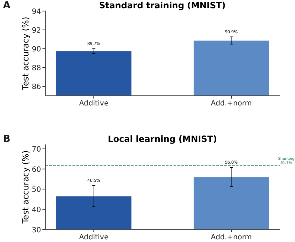
Figure S9: Additive + normalization control (MNIST stress-regime diagnostic). (A) Standard backprop: normalization provides a small boost (89.7% \rightarrow 90.9%). (B) Local learning: normalization improves additive from 46.5% to 56.0% (+9.5 pp), partially closing the gap to shunting (61.7%, dashed green). These lower local accuracies come from a separate stress-regime diagnostic, not from the matched-capacity performance setting in Table S3.
