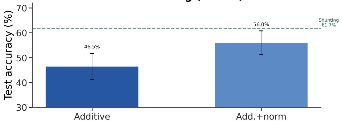
Figure S9: Additive + normalization control (MNIST stress-regime diagnostic). (A) Standard backprop: normalization provides a small boost (89.7% \rightarrow 90.9%). (B) Local learning: normalization improves additive from 46.5% to 56.0% (+9.5 pp), partially closing the gap to shunting (61.7%, dashed green). These lower local accuracies come from a separate stress-regime diagnostic, not from the matched-capacity performance setting in Table S3.
